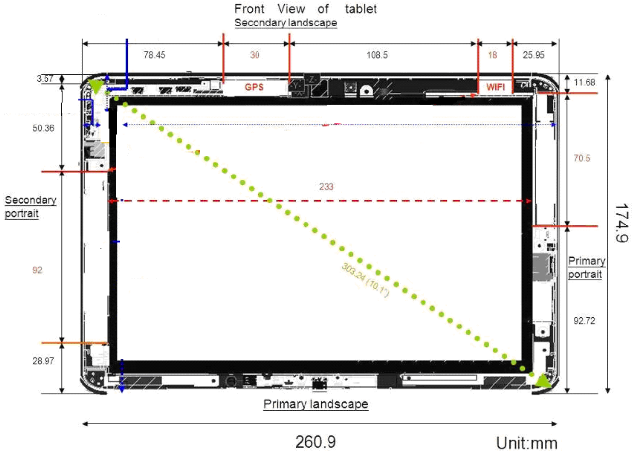
Fig.8 Antenna position of EUT
