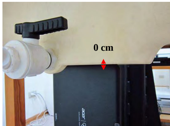
Fig.4 EUT Primary Portrait mode to flat phantom
