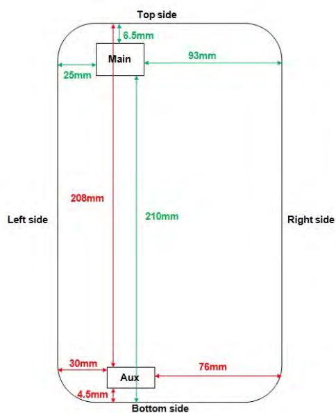
Fig.7 Antenna position of EUT (Back view)
