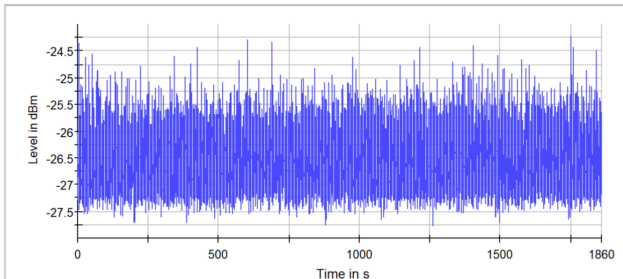
802.11a Channel 100
