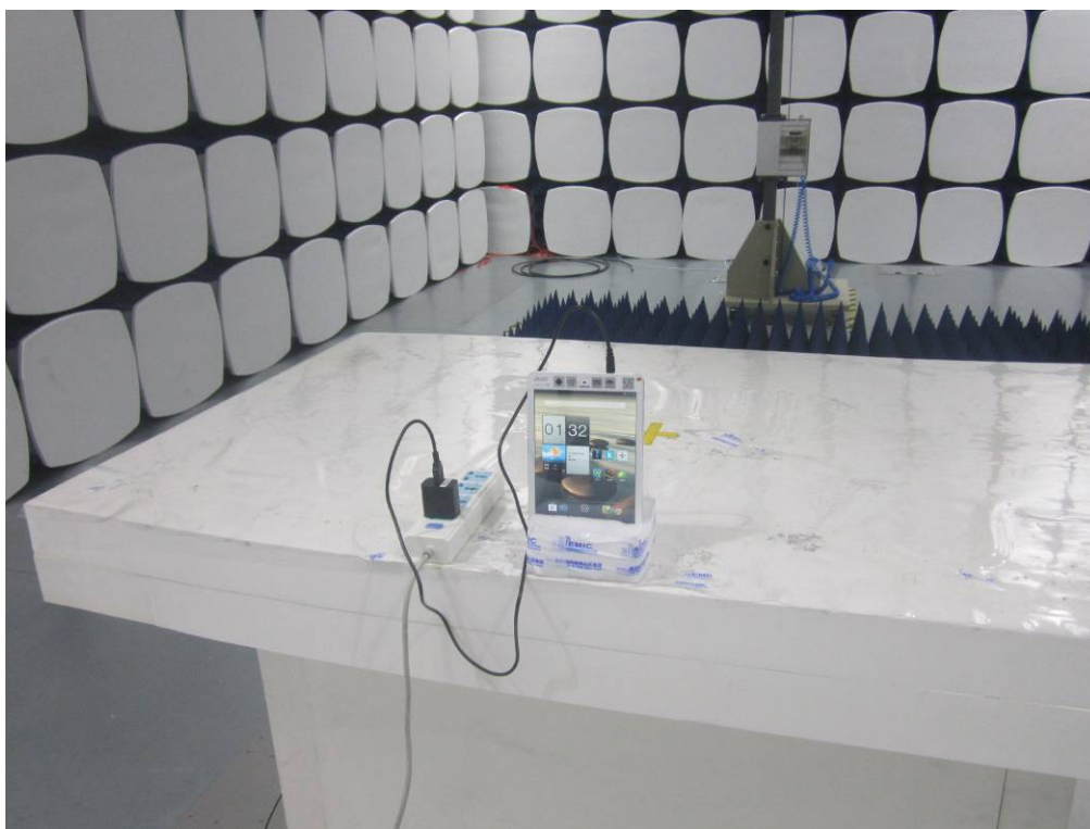
Radiated Spurious Emissions Test Setup Above 1GHz –Front View(Adapter1)
