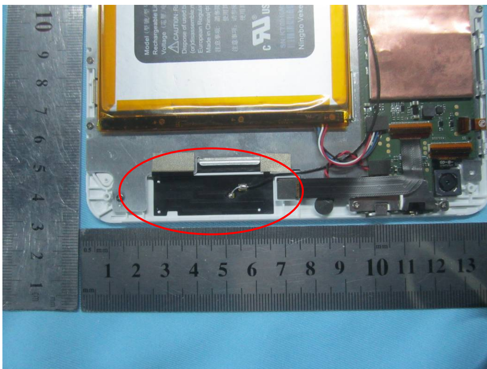
WIFI/Bluetooth Antenna View
