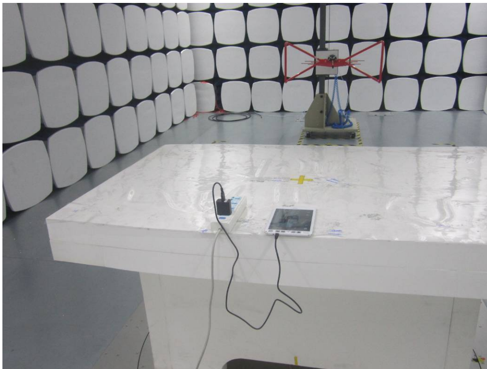
Radiated Spurious Emissions Test Setup Below 1GHz - Front View(Adapter1)
