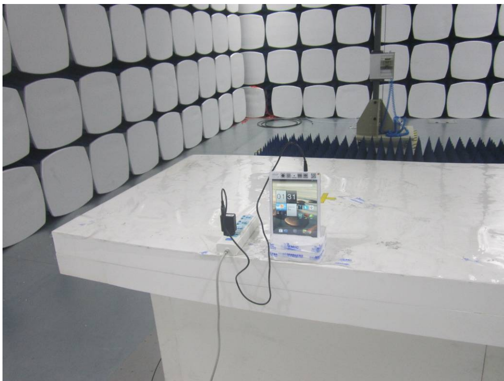
Radiated Spurious Emissions Test Setup Above 1GHz –Front View(Adapter2)
