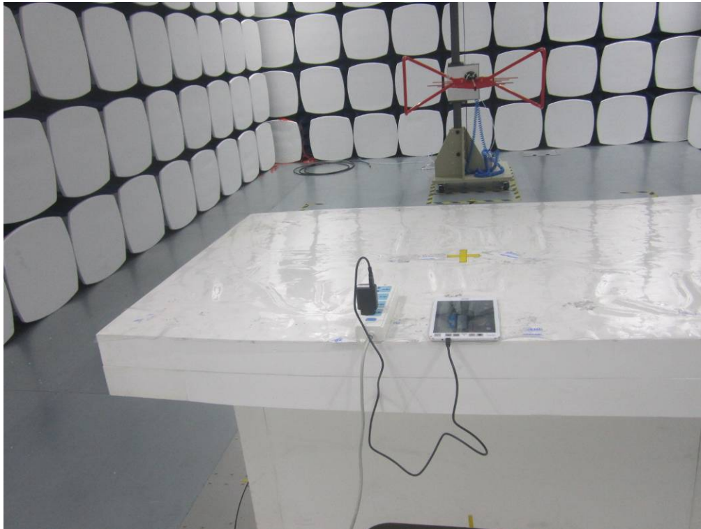
Radiated Spurious Emissions Test Setup Below 1GHz - Front View(Adapter2)
