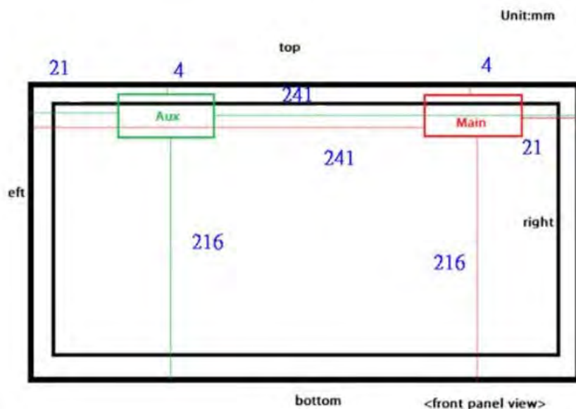
Fig.10 Antenna location of EUT
