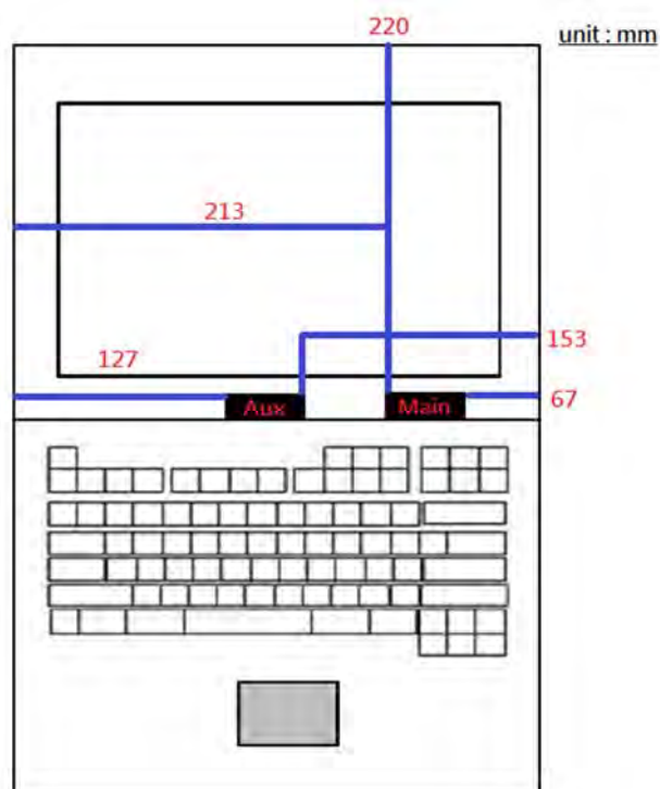
Fig.6 Antenna position of EUT
