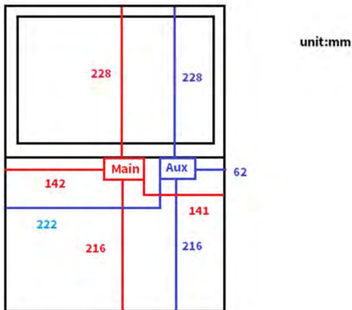
Fig.6 Antenna position of EUT
