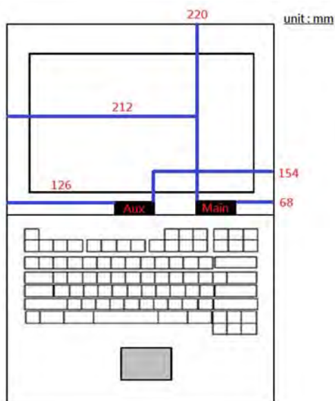
Fig.6 Antenna position of EUT
