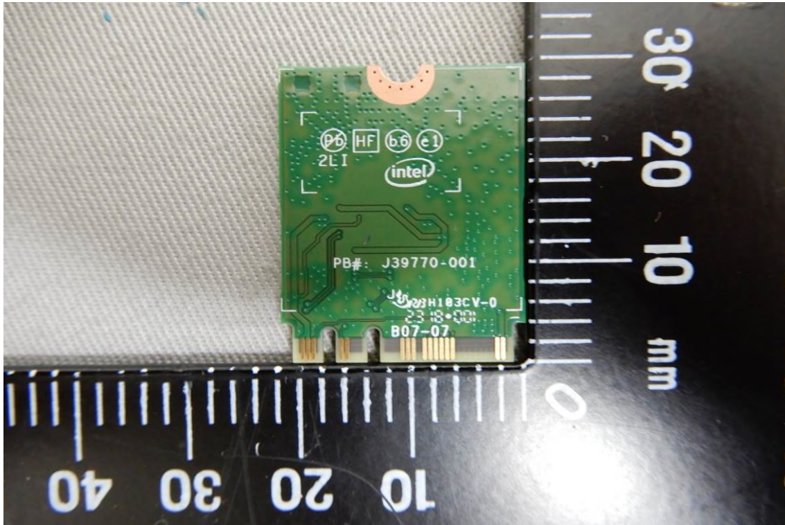
WLAN / BT Module - 3 (Model No.: 9260NGW)
