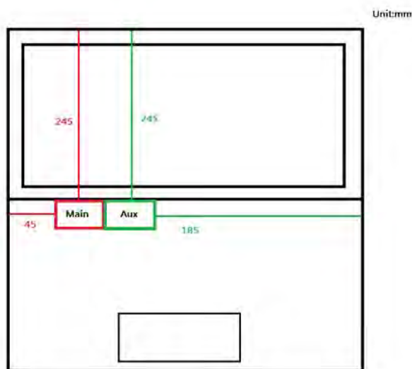
Fig.6 Antenna location (front view of laptop mode)
