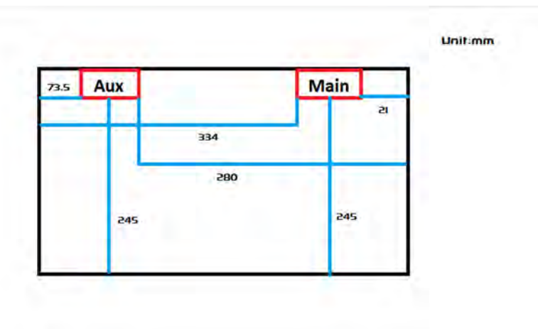
Fig.8 Antenna position of EUT
