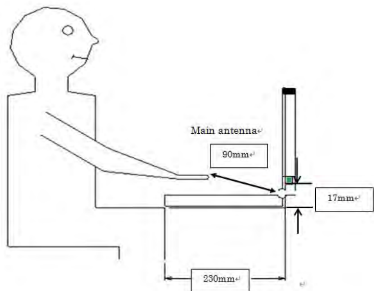
Fig.7 Antenna location of EUT (laptop mode)
