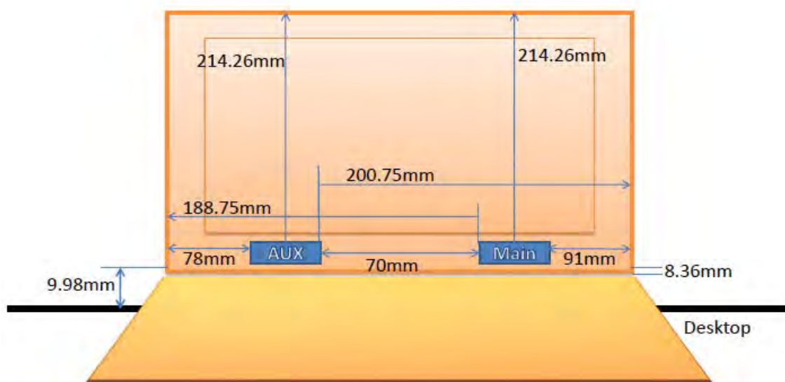
Front view
