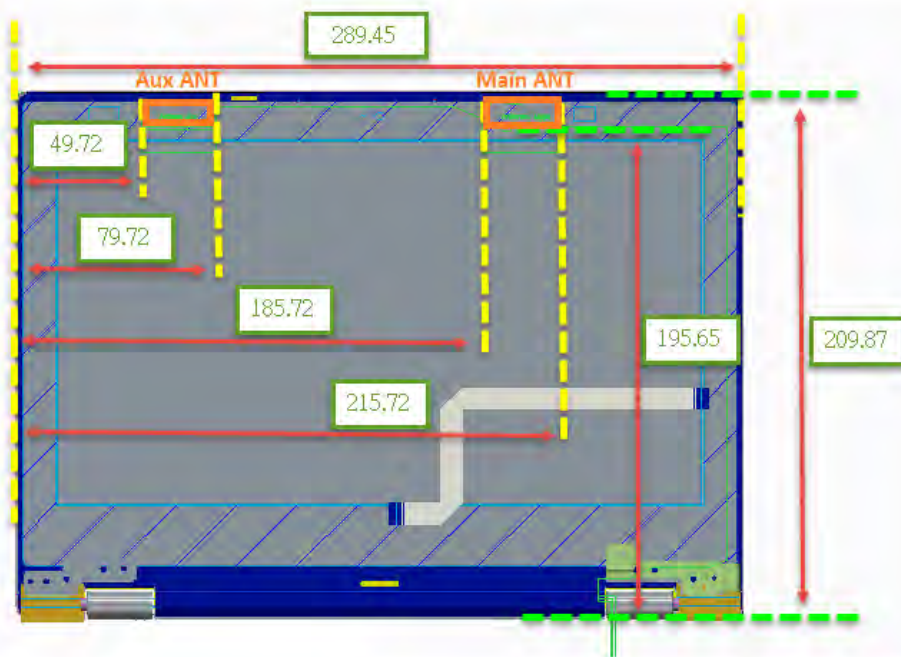
Fig.7 Antenna position of EUT (Front view)
