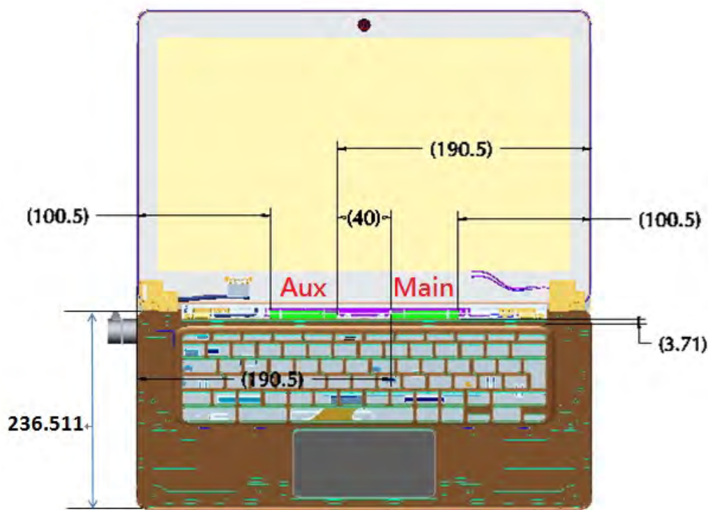
Fig.6 Antenna position of EUT (Front view)
