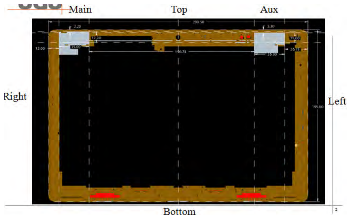
Fig.9 Antenna position of EUT (Back view)
