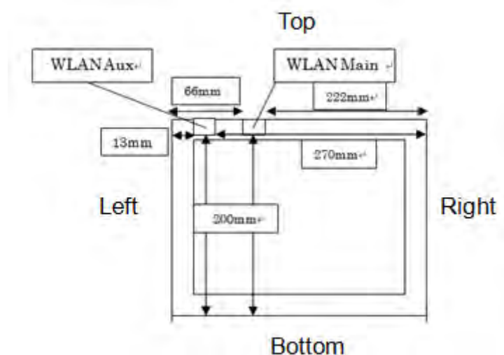
Fig.10 Antenna position of EUT (front view of tablet mode)
