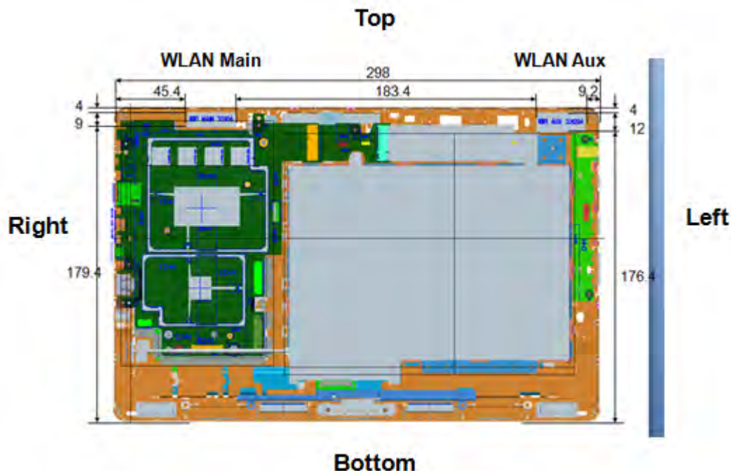
Fig.9 Antenna position of EUT (Back view)
