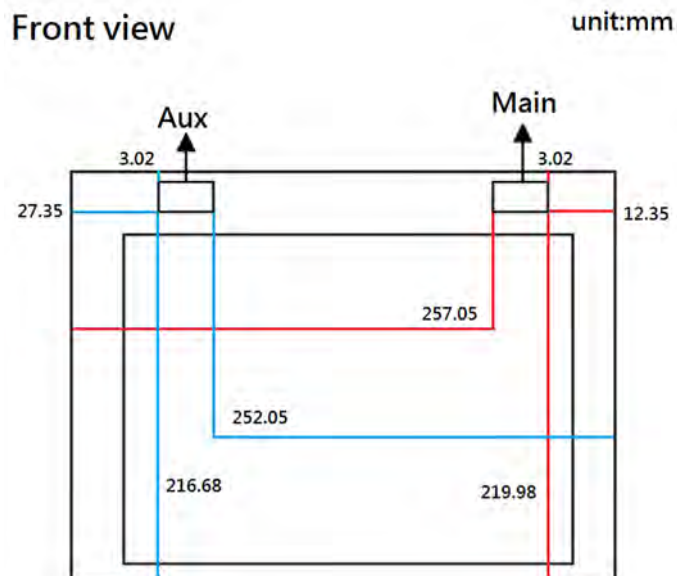
Fig.8 Antenna position of EUT (Front view)
