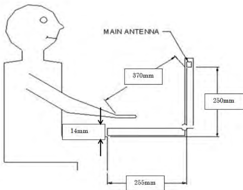
Fig.13 Antenna location of EUT (laptop mode)
