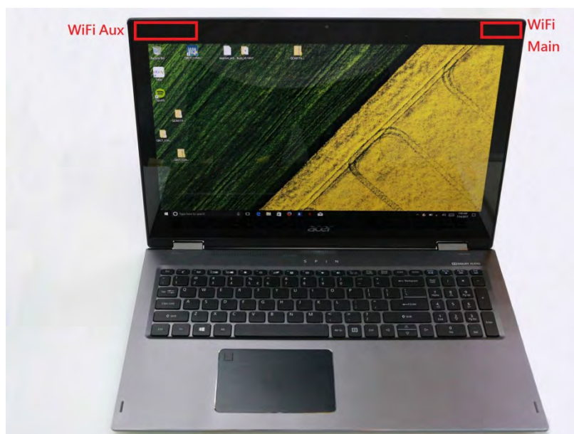
Fig.9 EUT (Open Mode)
