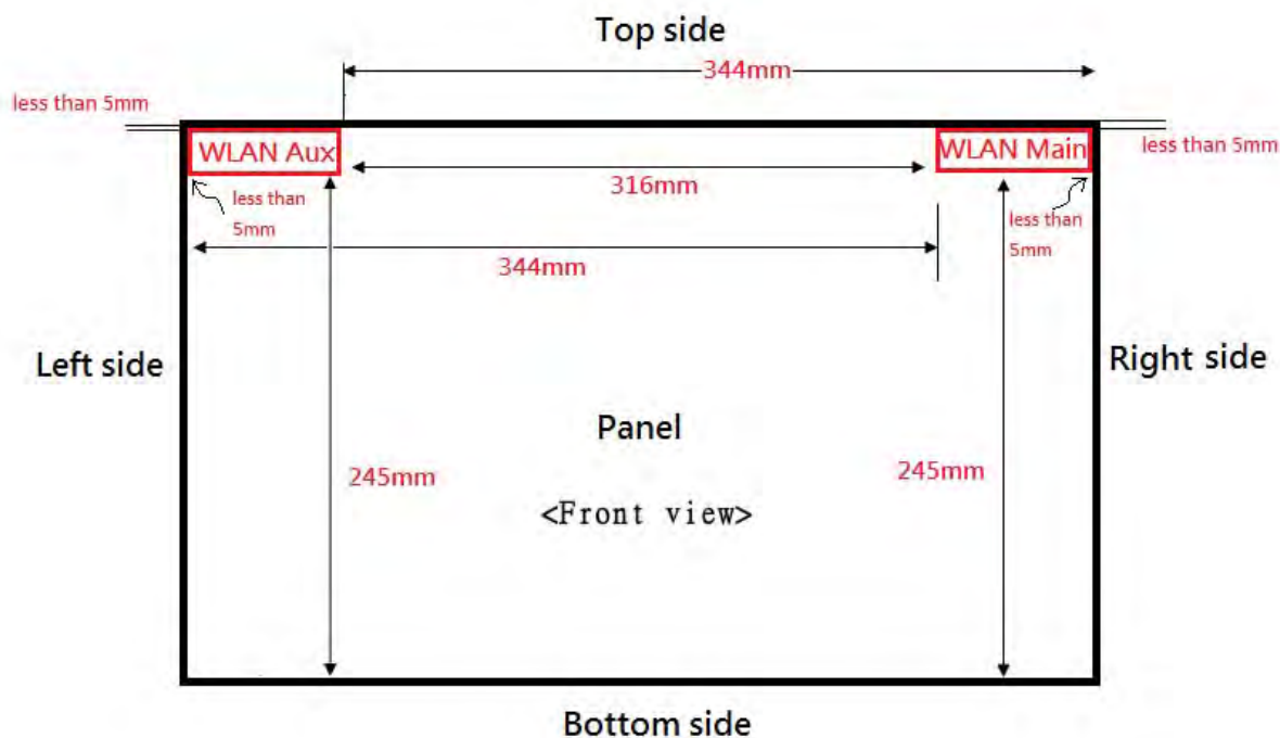
Fig.11 Antenna location of EUT (tablet mode)
