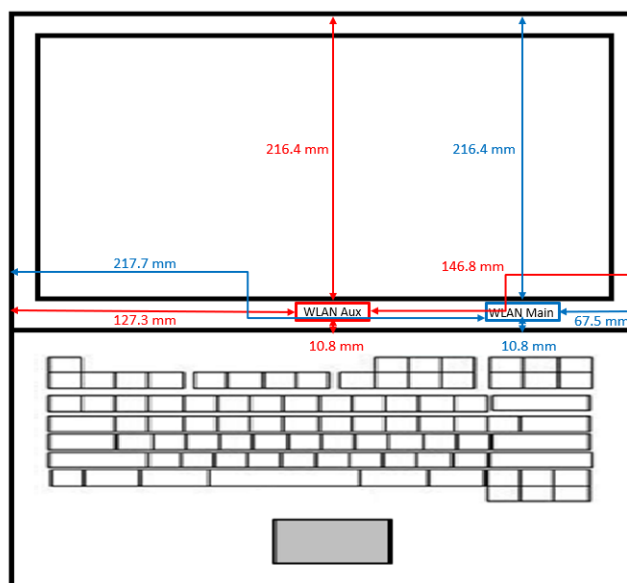
Photograph 5. Antenna position of EUT
