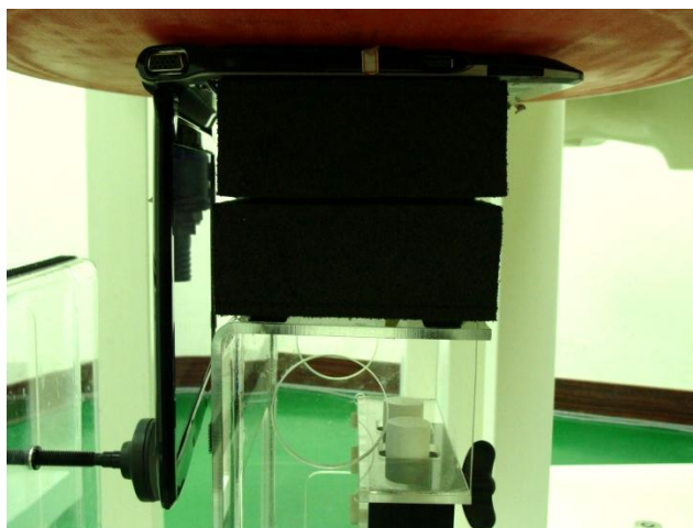
Bottom of the Laptop with Phantom 0 cm Gap
