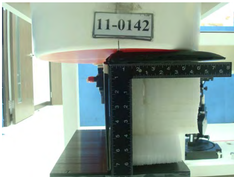
Figure 1. Body SAR Test Setup (Bottom Close Body)
