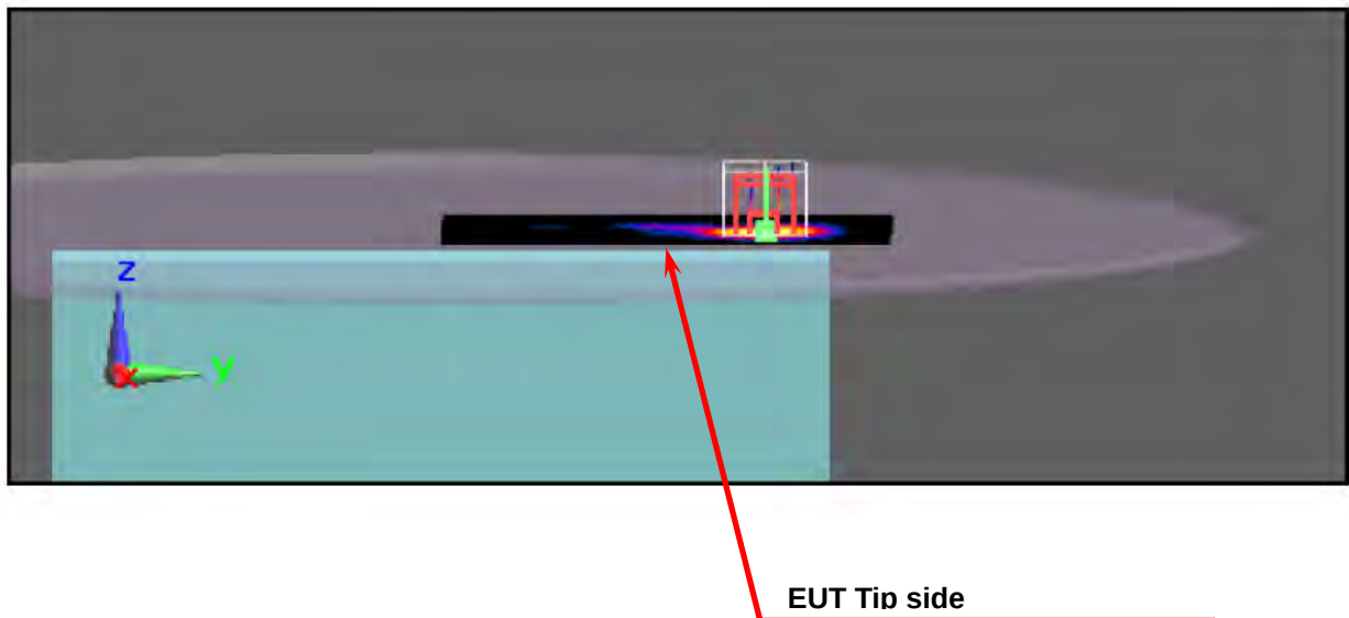
Figure 1. Body SAR Test Setup (Flat Section)_ Tablet Mode LCD Tip Close Body
