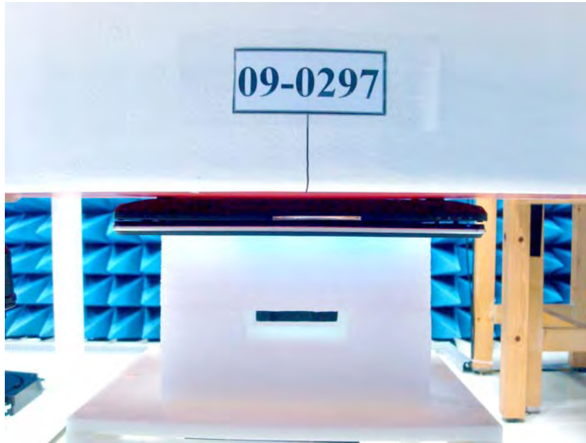
Figure 2. Body SAR Test Setup (Flat Section) _Tablet Mode Bottom Close Body
