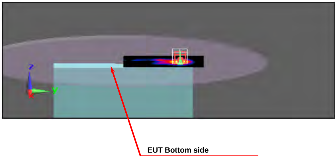
Figure 2. Body SAR Test Setup (Flat Section) _Tablet Mode Bottom Close Body
