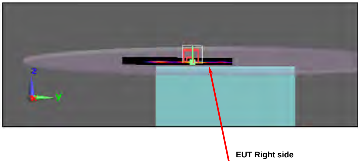
Figure 3. Body SAR Test Setup (Flat Section)_ Tablet Mode LCD Right side Close Body
