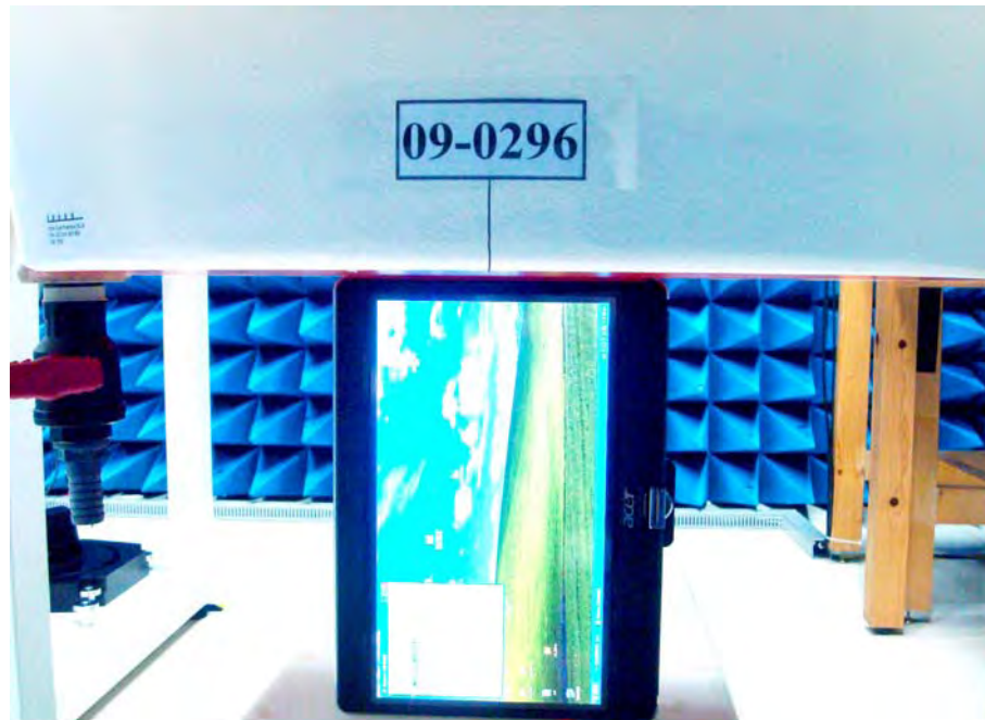
Figure 3. Body SAR Test Setup (Flat Section)_ Tablet Mode LCD Right side Close Body
