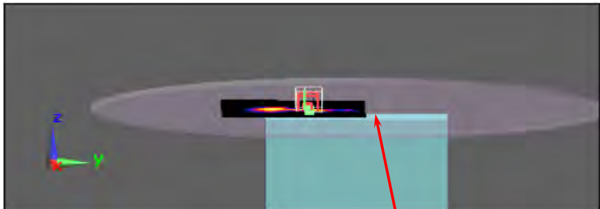
Figure 3. Body SAR Test Setup (Flat Section)_ Tablet Mode LCD Right side Close Body
