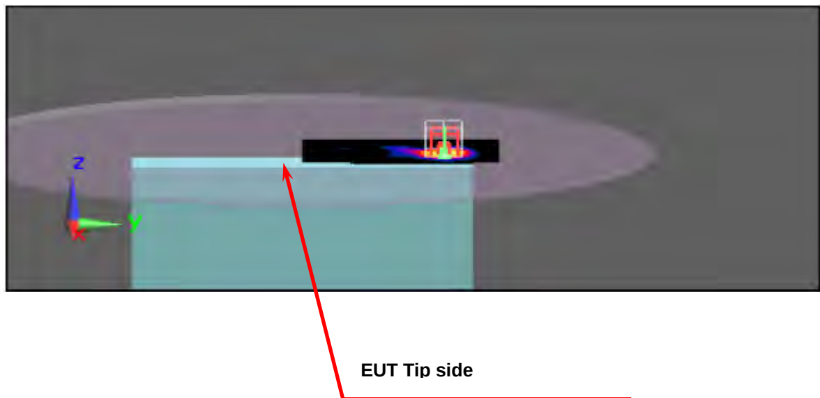
Figure 1. Body SAR Test Setup (Flat Section)_ Tablet Mode LCD Tip Close Body
