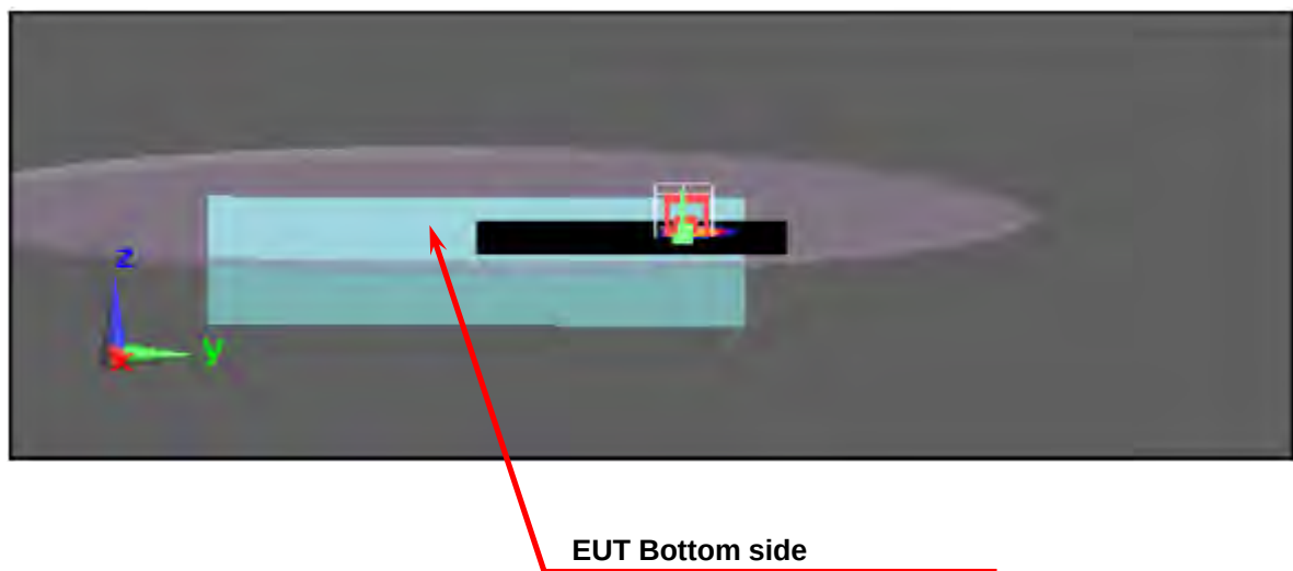
Figure 2. Body SAR Test Setup (Flat Section) _Tablet Mode Bottom Close Body
