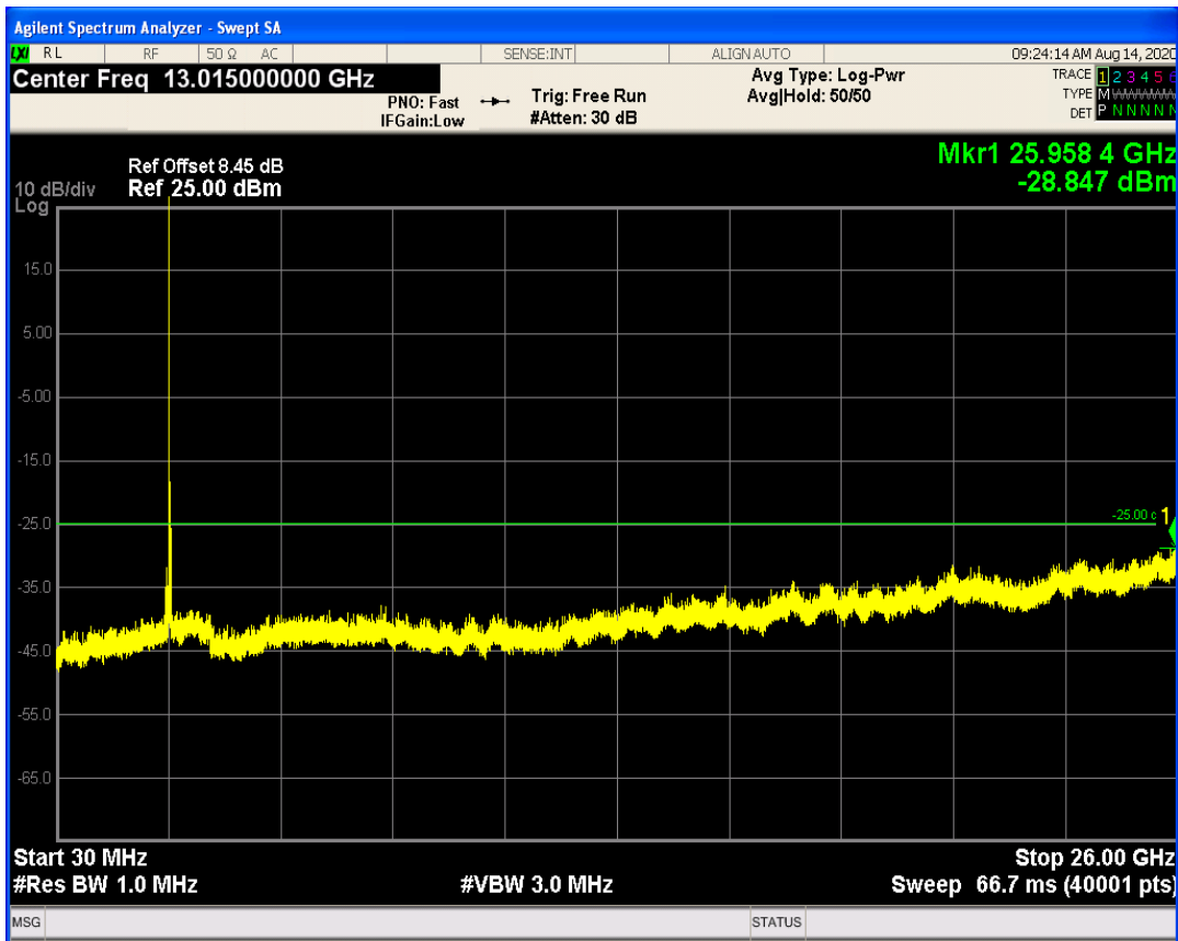
LTE Band41 QPSK BW=20MHz Channel=41140 RB Size=100 Position=#0
