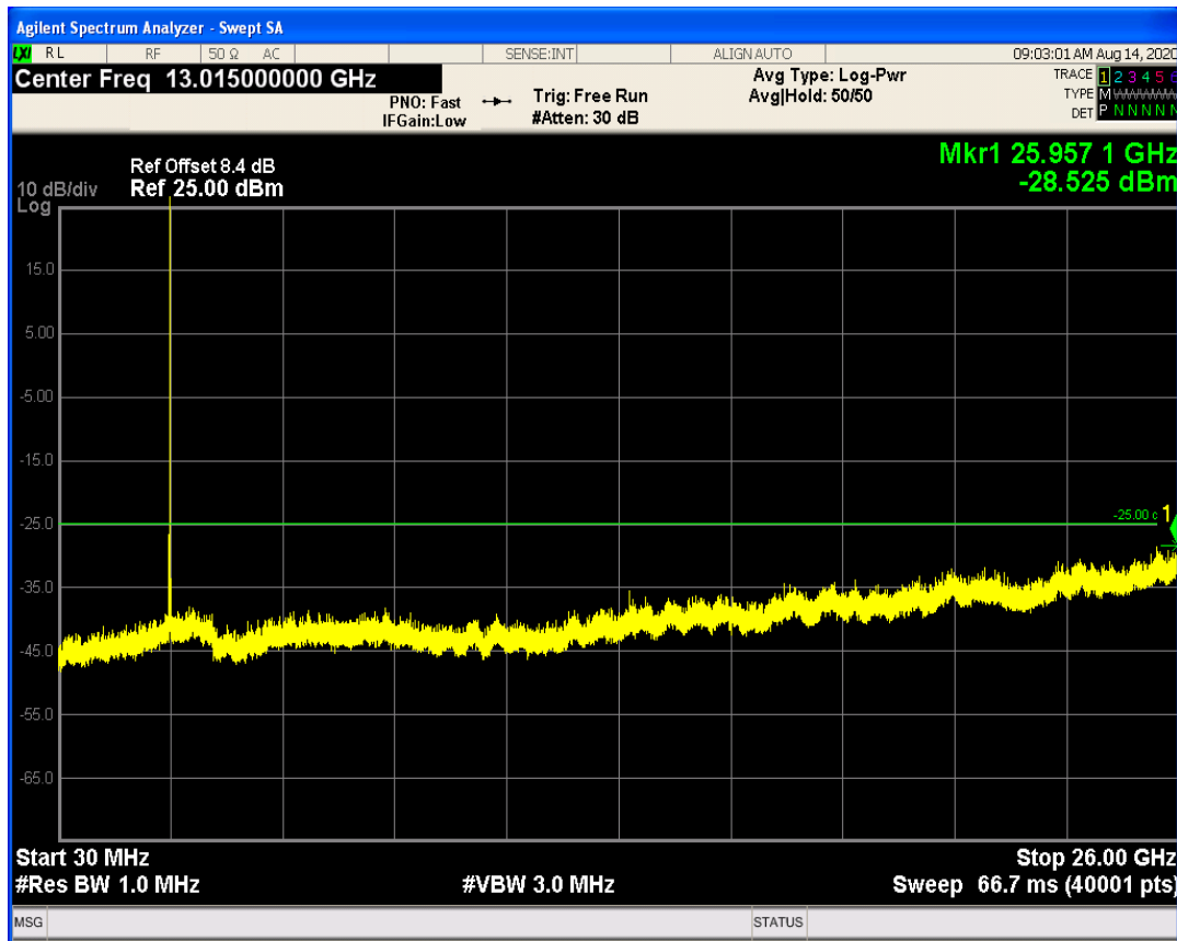
LTE Band41 QPSK BW=5MHz Channel=40740 RB Size=25 Position=#0
