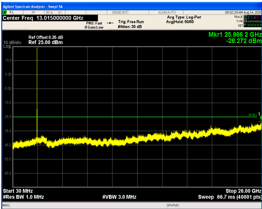
LTE Band41 QPSK BW=5MHz Channel=40740 RB Size=1 Position=#0
