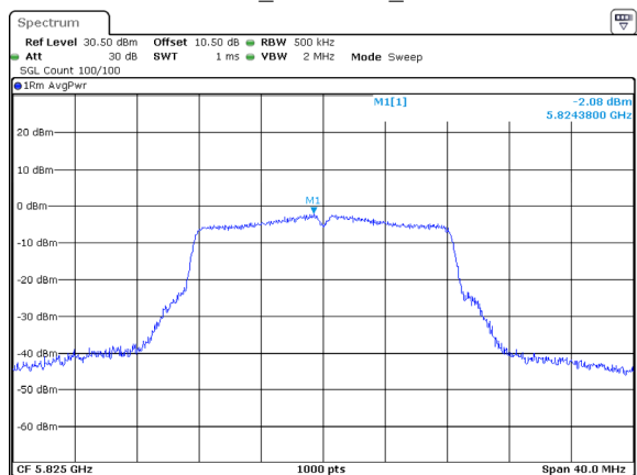
802.11a_5825MHz_ANT2
