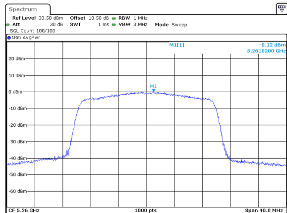
802.11ax20_5260MHz_RU_Full_ANT2
