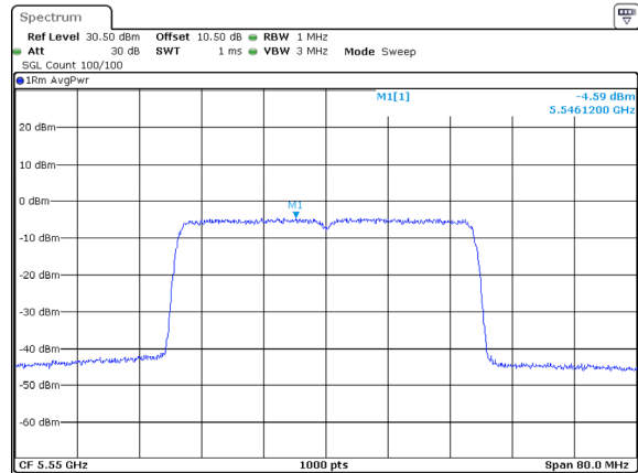
802.11ax40_5550MHz_RU_Full_ANT1
