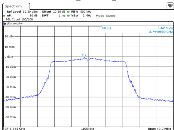
802.11ac20_5745MHz_ANT1
