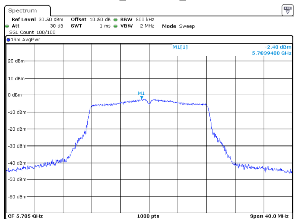
802.11a_5785MHz_ANT2
