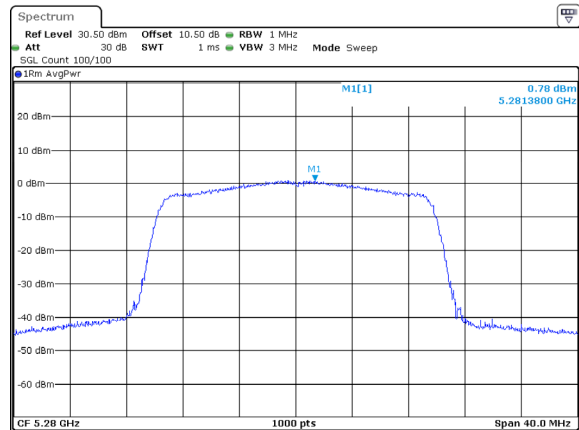
802.11ax20_5280MHz_RU_Full_ANT1
