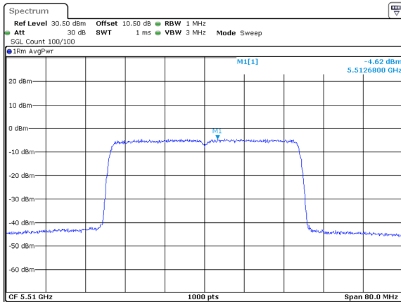
802.11ax40_5510MHz_RU_Full_ANT1
