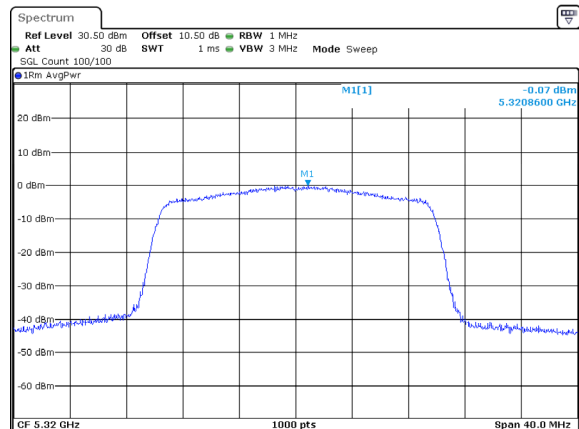
802.11ax20_5320MHz_RU_Full_ANT2
