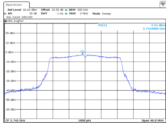
802.11ac20_5745MHz_ANT2
