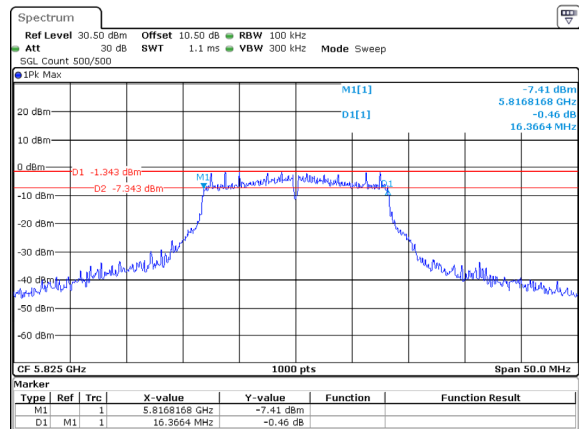
802.11a_5825MHz_ANT2
