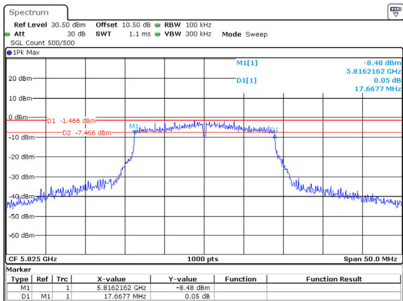
802.11ac20_5825MHz_ANT2
