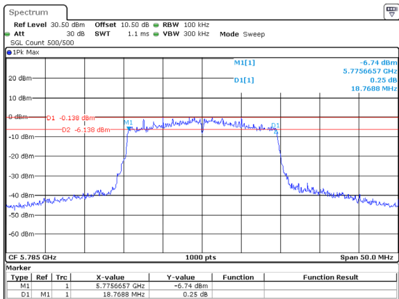
802.11ax20_5785MHz_RU_Full_ANT1
