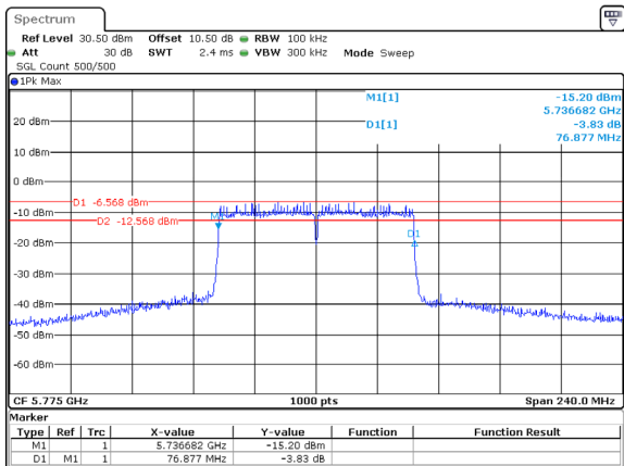
802.11ac80_5775MHz_ANT2
