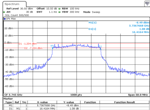
802.11a_5745MHz_ANT2
