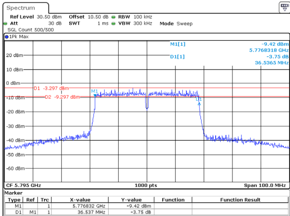
802.11ac40_5795MHz_ANT2
