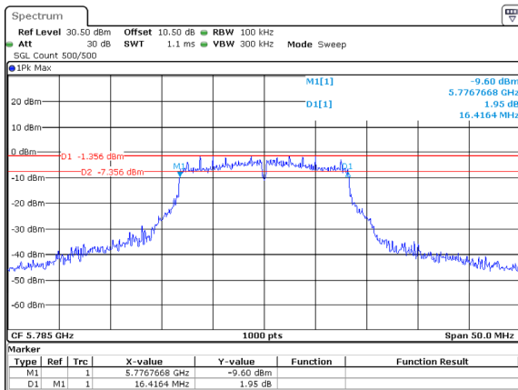
802.11a_5785MHz_ANT2
