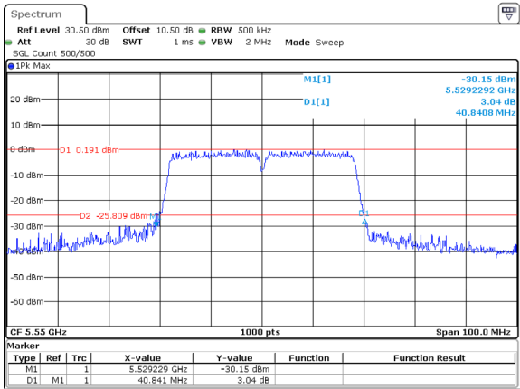
802.11ac40_5550MHz_ANT2
