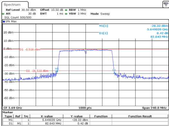
802.11ac80_5690MHz_ANT2
