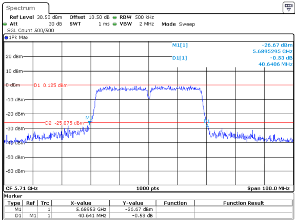
802.11ac40_5710MHz_ANT2
