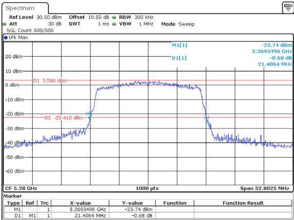
802.11ax20_5280MHz_RU_Full_ANT2
