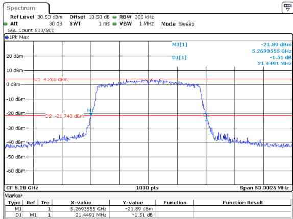
802.11ax20_5280MHz_RU_Full_ANT1
