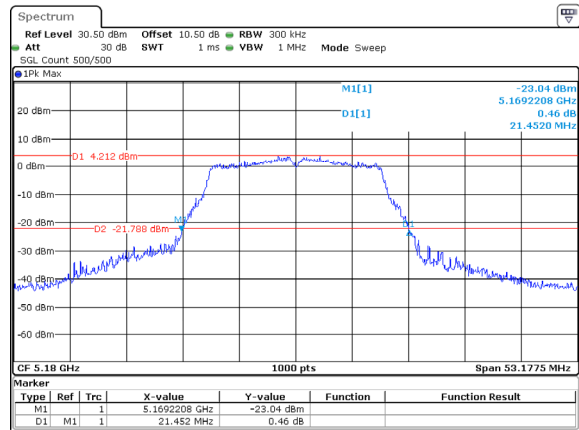
802.11a_5180MHz_ANT2
