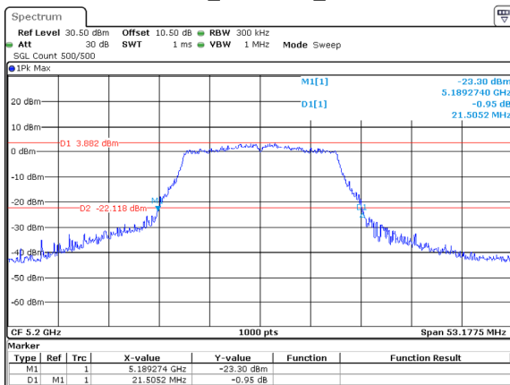
802.11a_5200MHz_ANT2
