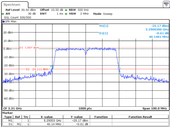
802.11ac40_5310MHz_ANT2
