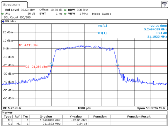
802.11ax20_5260MHz_RU_Full_ANT1
