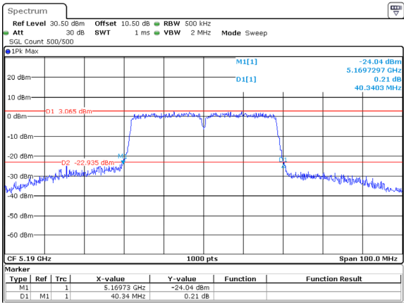
802.11ac40_5190MHz_ANT2
