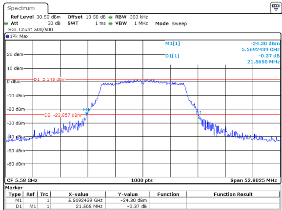
802.11a_5580MHz_ANT2
