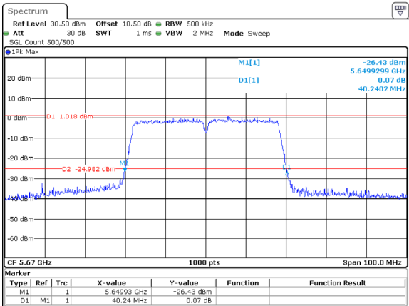
802.11ac40_5670MHz_ANT1
