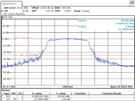
802.11a_5700MHz_ANT2
