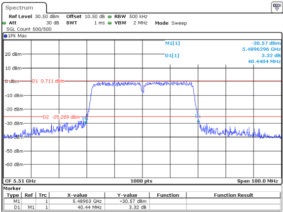
802.11ac40_5510MHz_ANT2
