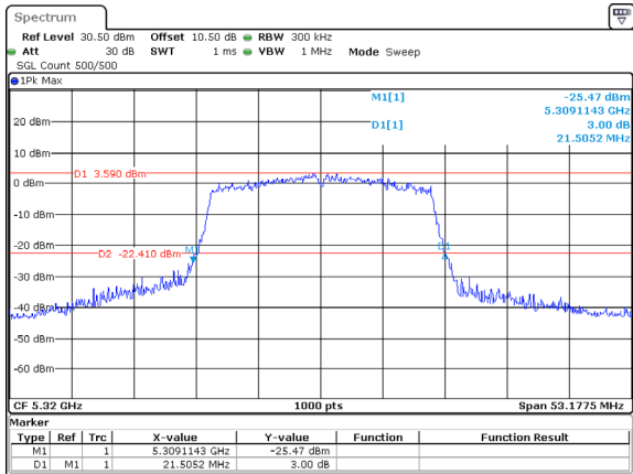
802.11ax20_5320MHz_RU_Full_ANT2
