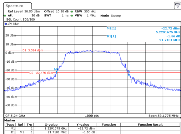
802.11a_5240MHz_ANT2
