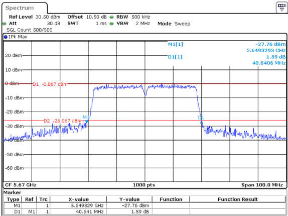
802.11ac40_5670MHz_ANT2
