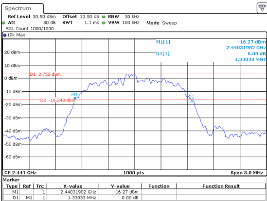
2DH1_Middle 1.330MHz
