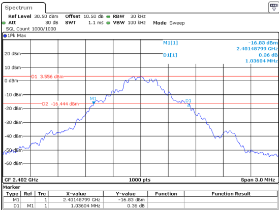
DH1_Low 1.036MHz
