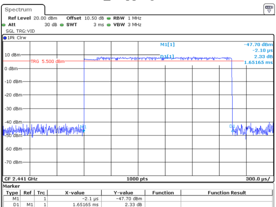
2DH3_Hopping 1.652ms
