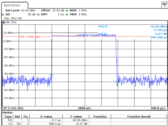
2DH1_Hopping 0.398ms
