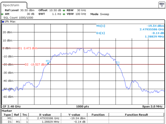
3DH1_High 1.288MHz
