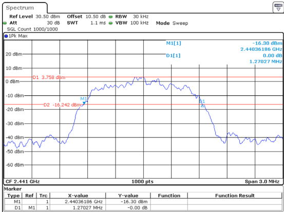
3DH1_Middle 1.270MHz
