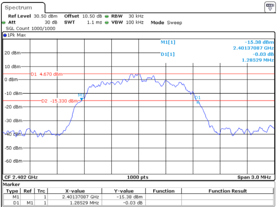
3DH1_Low 1.285MHz
