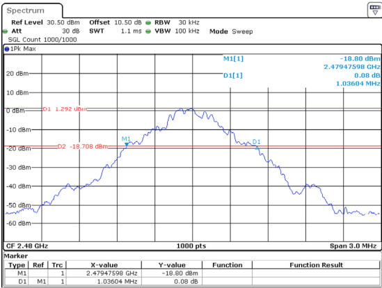
DH1_High 1.036MHz
