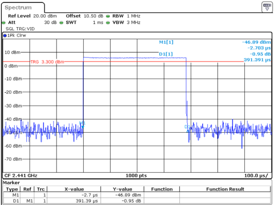
DH1_Hopping 0.391ms
