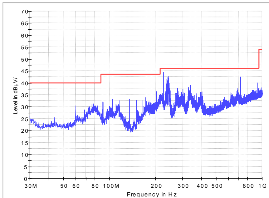
Field strength 30M-1GHz 1F 3m chamber
