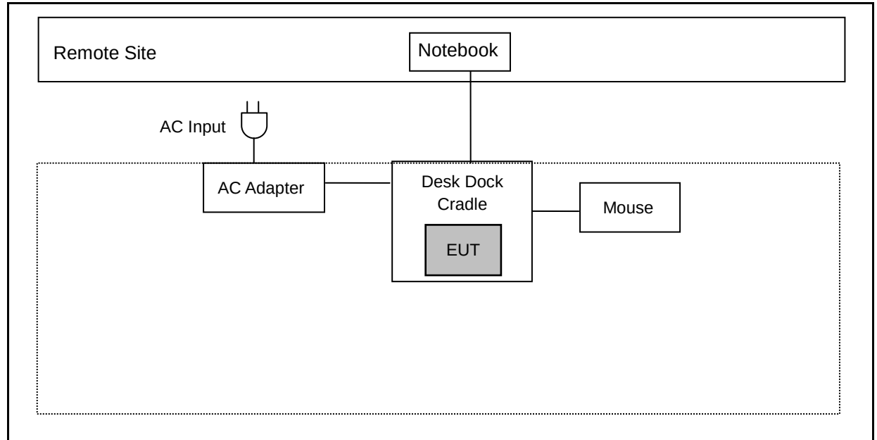
Conducted Emissions
