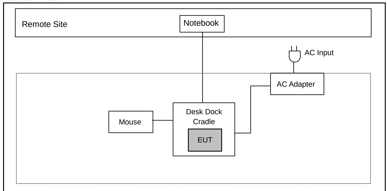
Radiated Emission
