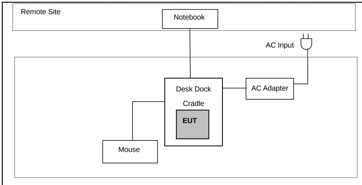
Radiated Emissions
