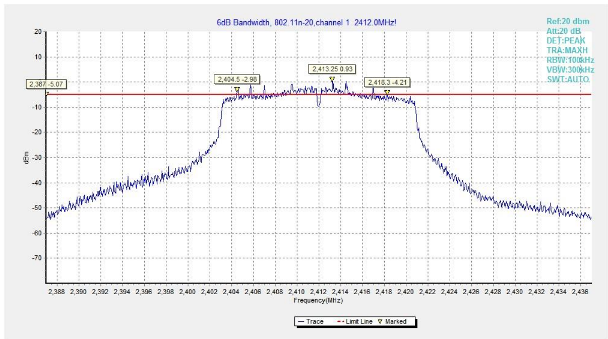
Fig.25 6dB Bandwidth (802.11n HT20, CH 1)
