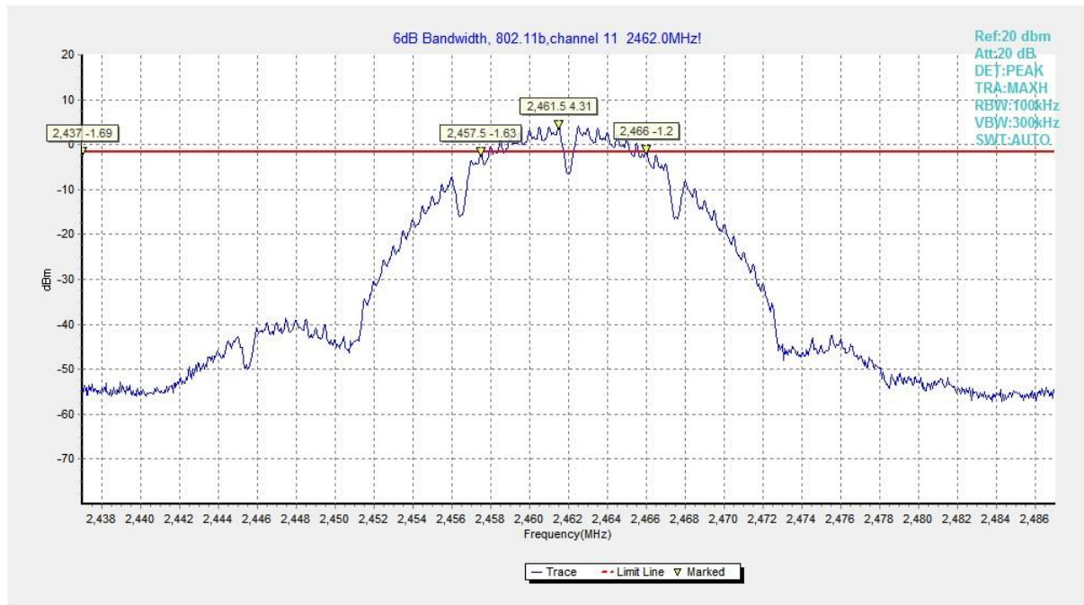
Fig.21 6dB Bandwidth (802.11b, CH 11)
