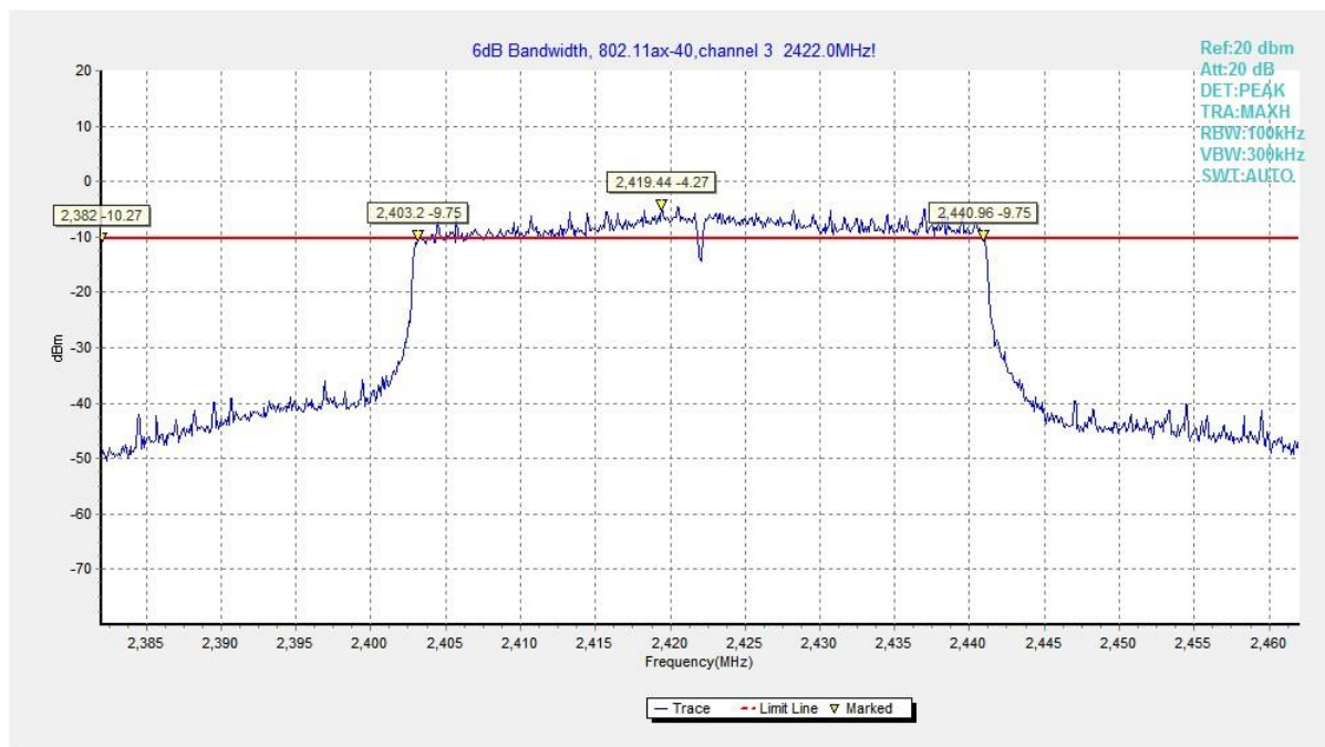
Fig.34 6dB Bandwidth (802.11ax HE40, CH 3)
