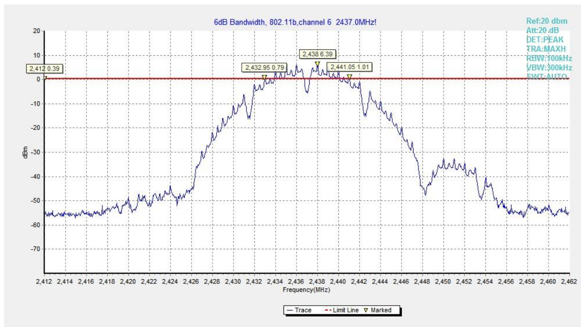
Fig.20 6dB Bandwidth (802.11b, CH 6)
