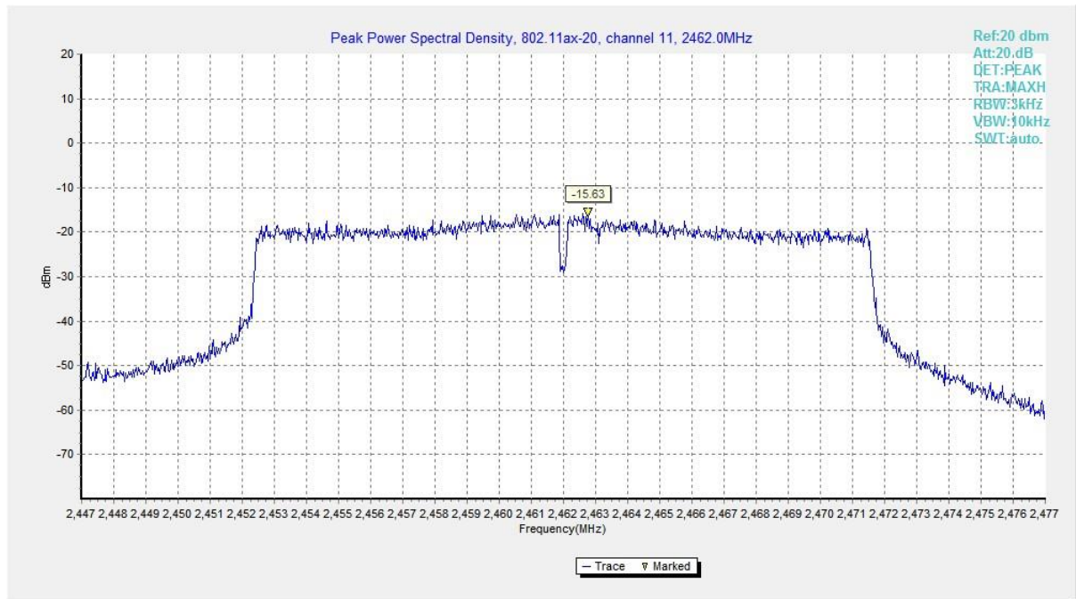
Fig.15 Power Spectral Density (802.11ax HE20, CH 11)
