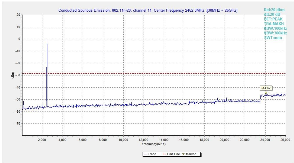
Fig.57 Conducted Spurious Emission (802.11n HT20, CH11)
