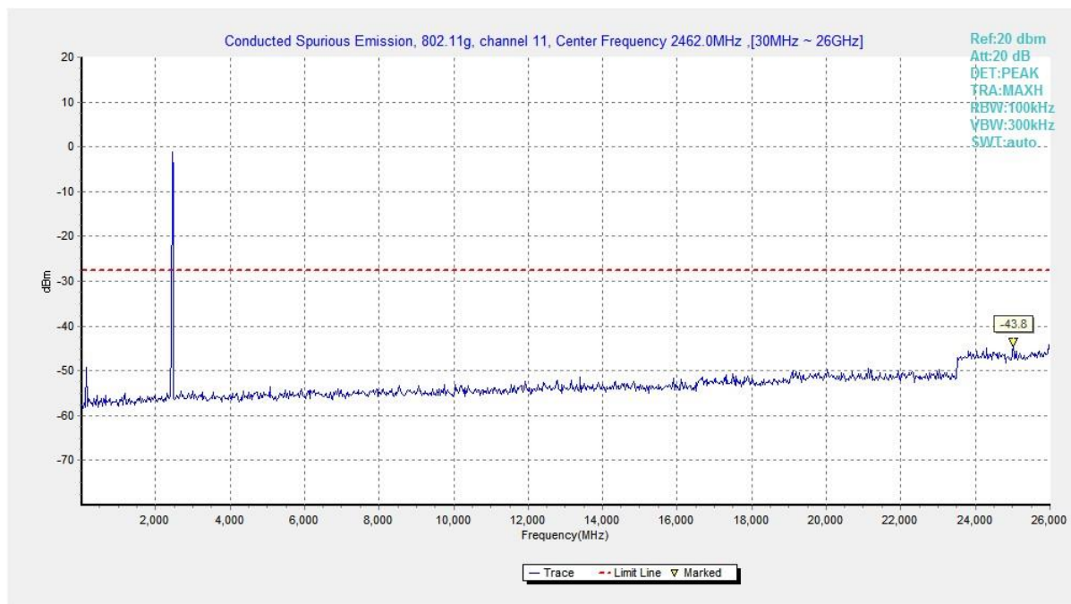
Fig.54 Conducted Spurious Emission (802.11g, CH11)
