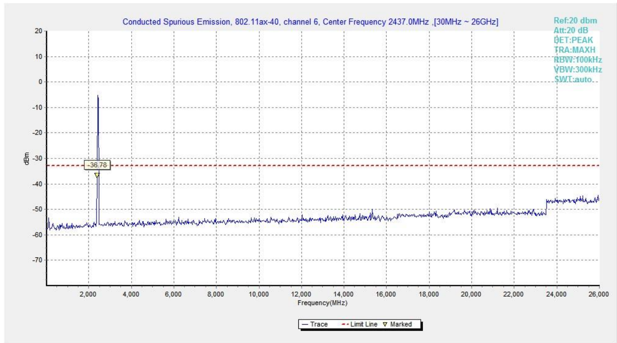
Fig.65 Conducted Spurious Emission (802.11ax HE40, CH6)
