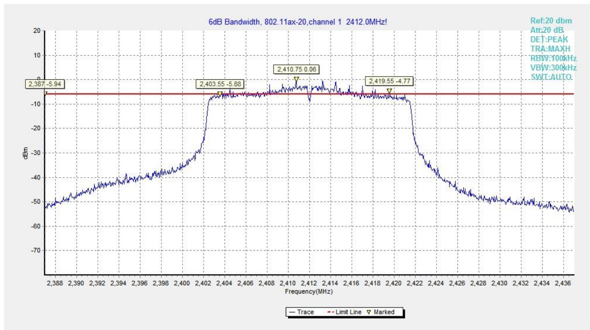
Fig.31 6dB Bandwidth (802.11ax HE20, CH 1)
