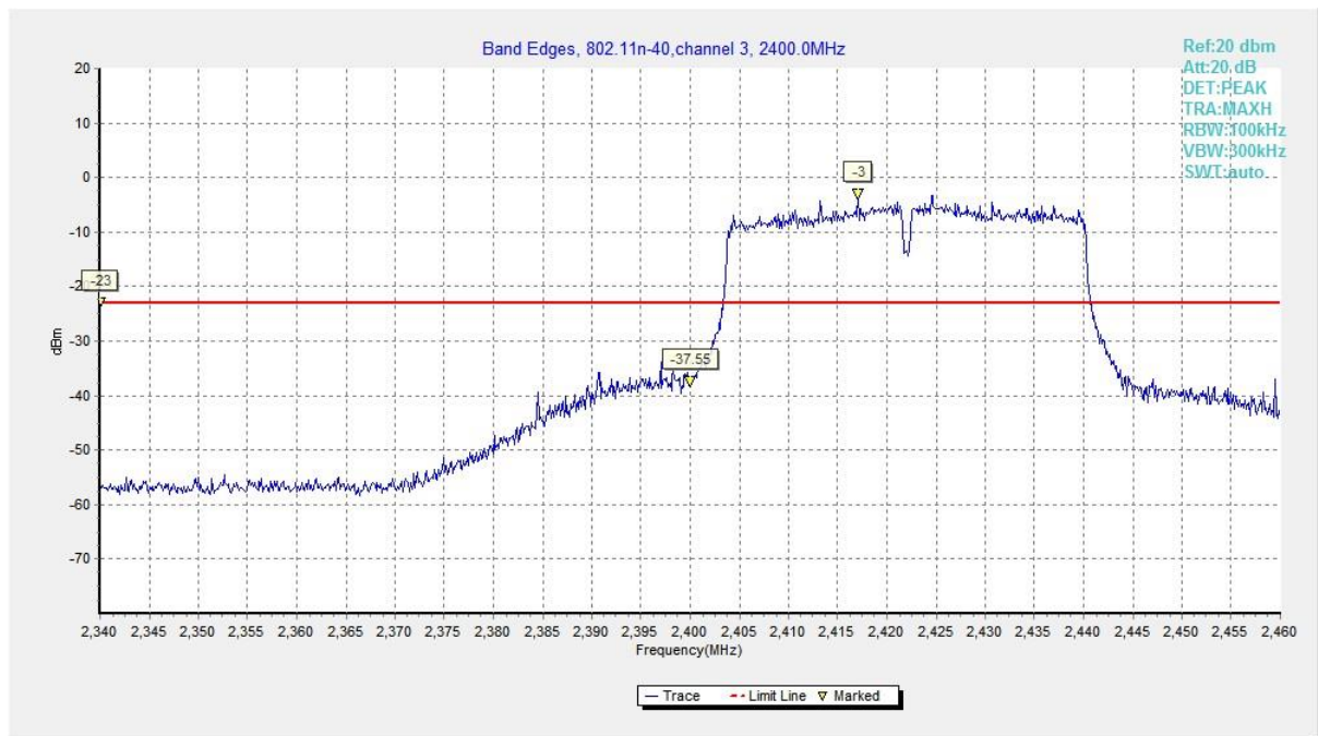
Fig.43 Band Edges (802.11n HT40, CH 3)
