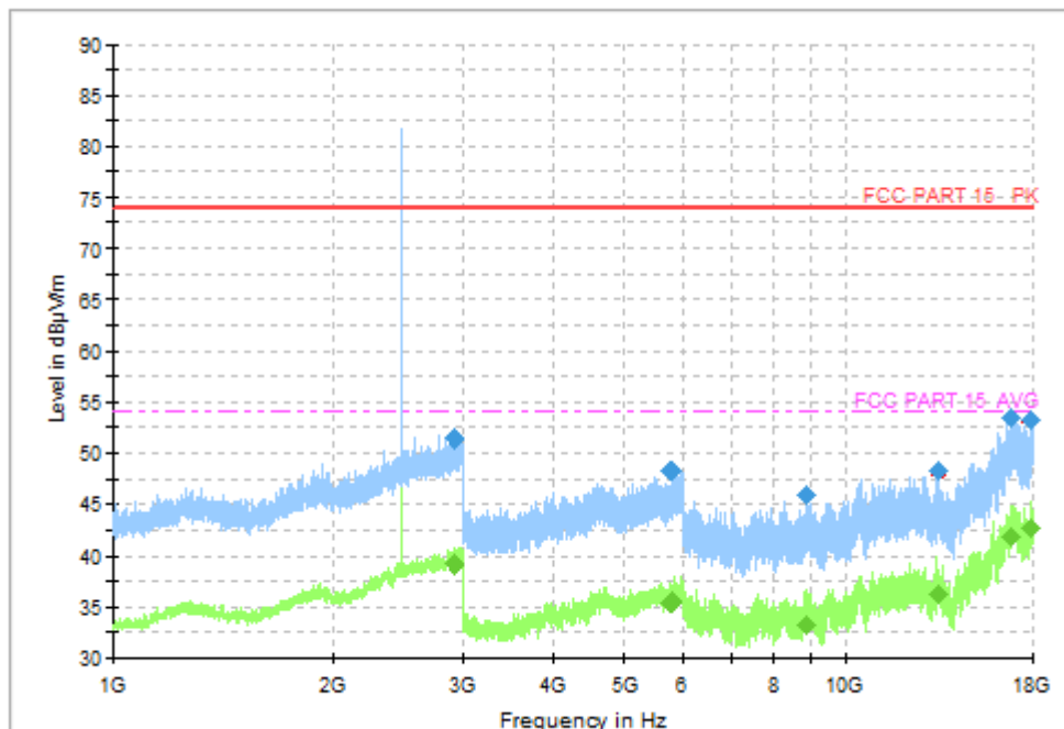
Fig.38 Radiated Spurious Emission (Ch39, 1 GHz - 18 GHz), 1M
