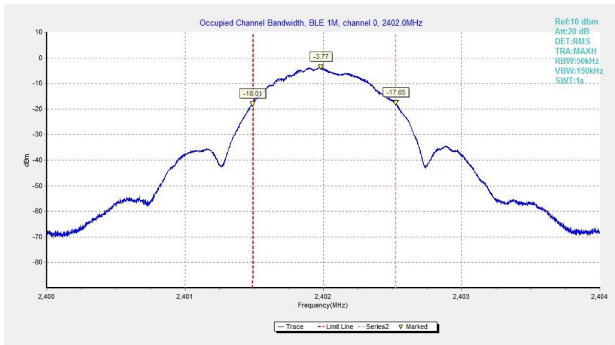
Fig.51 99% Occupied Bandwidth (Ch 0), LE 1M
