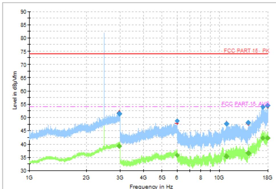
Fig.46 Radiated Spurious Emission (Ch39, 1 GHz - 18 GHz), 2M
