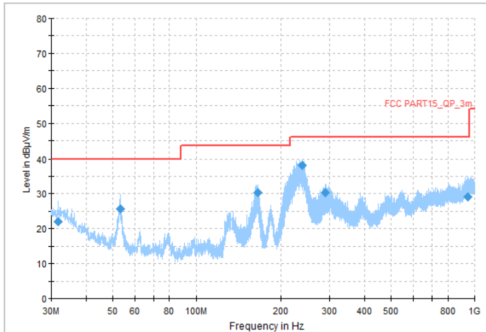
Fig.35 Radiated Spurious Emission (Ch19, 30 MHz - 1 GHz), 1M
