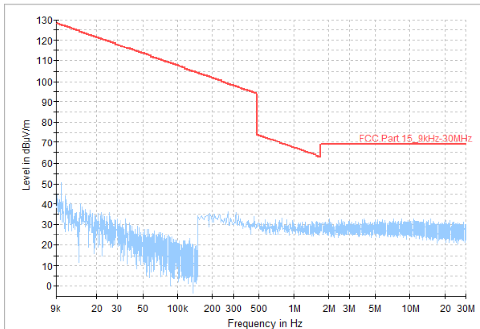
Fig.34 Radiated Spurious Emission (Ch19, 9 kHz - 30 MHz), 1M
