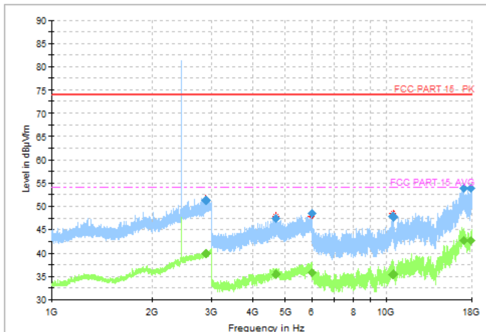
Fig.36 Radiated Spurious Emission (Ch19, 1 GHz - 18 GHz), 1M
