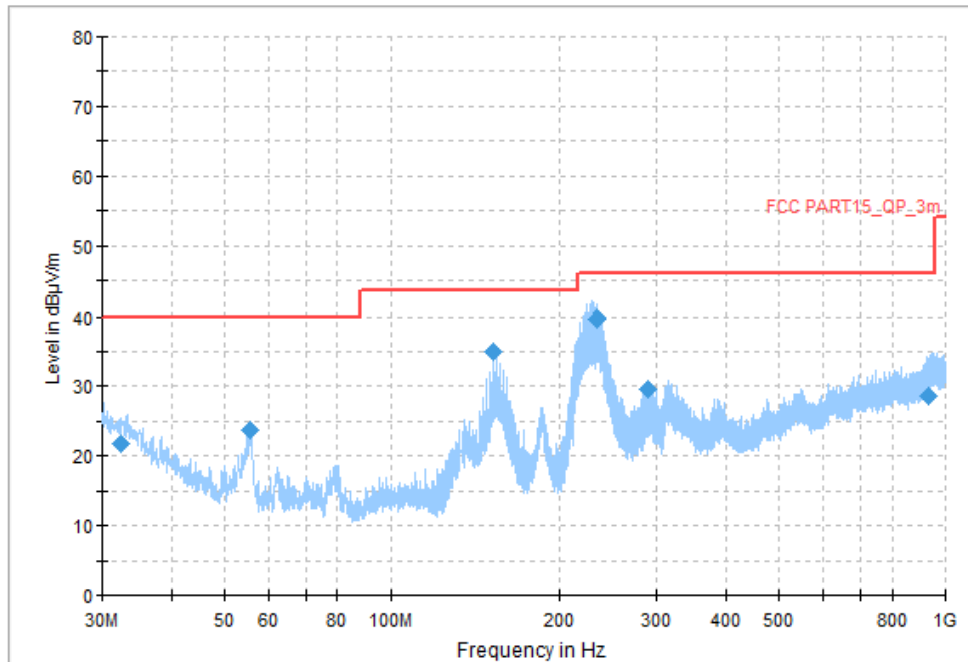
Fig.43 Radiated Spurious Emission (Ch19, 30 MHz - 1 GHz), 2M
