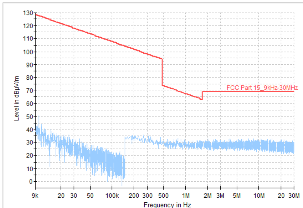
Fig.42 Radiated Spurious Emission (Ch19, 9 kHz - 30 MHz), 2M
