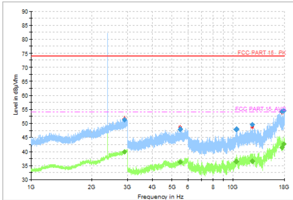
Fig.33 Radiated Spurious Emission (Ch0, 1 GHz - 18 GHz), 1M
