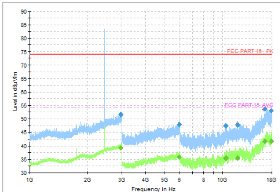
Fig.44 Radiated Spurious Emission (Ch19, 1 GHz - 18 GHz), 2M
