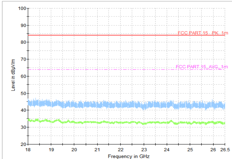
Fig.45 Radiated Spurious Emission (Ch19, 18 GHz - 26.5 GHz), 2M
