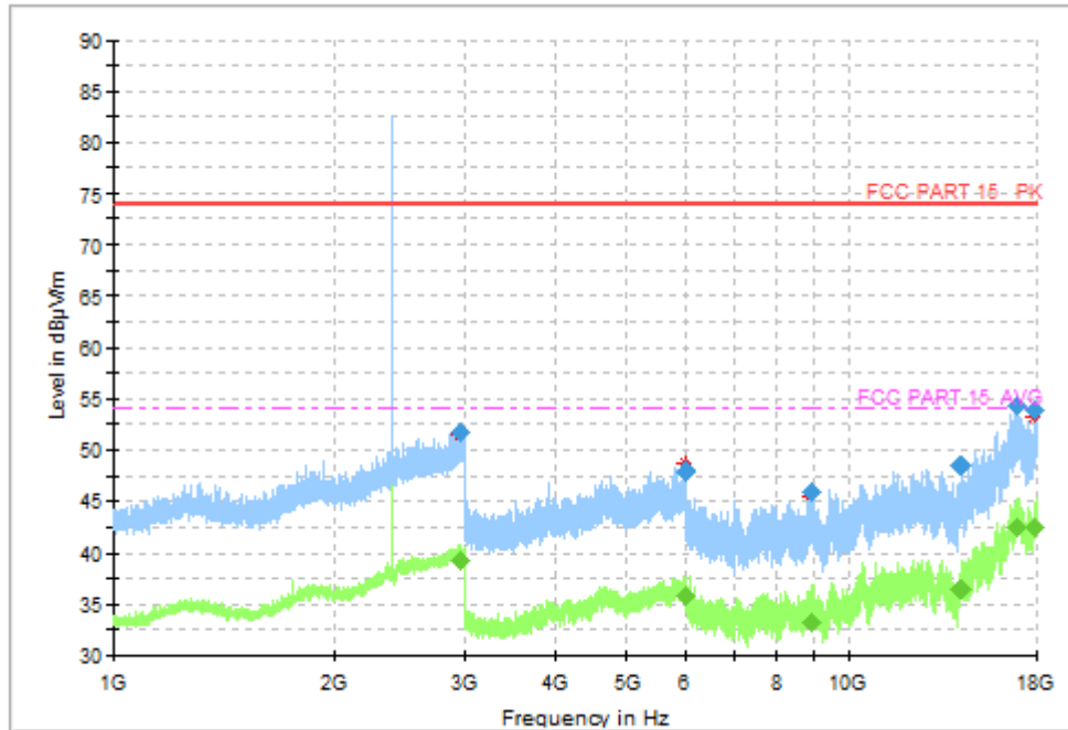
Fig.41 Radiated Spurious Emission (Ch0, 1 GHz - 18 GHz), 2M
