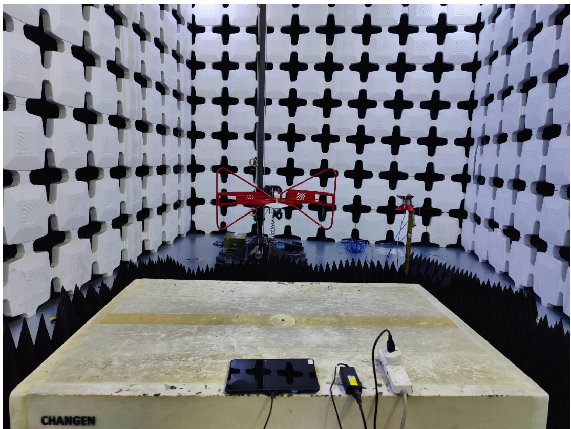
1. Radiated Emissions (Part 15B Camera, 30MHz-1GHz)
