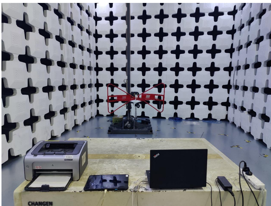
5. Radiated Emissions (Part 15B Data Transfer, 30MHz-1GHz)
