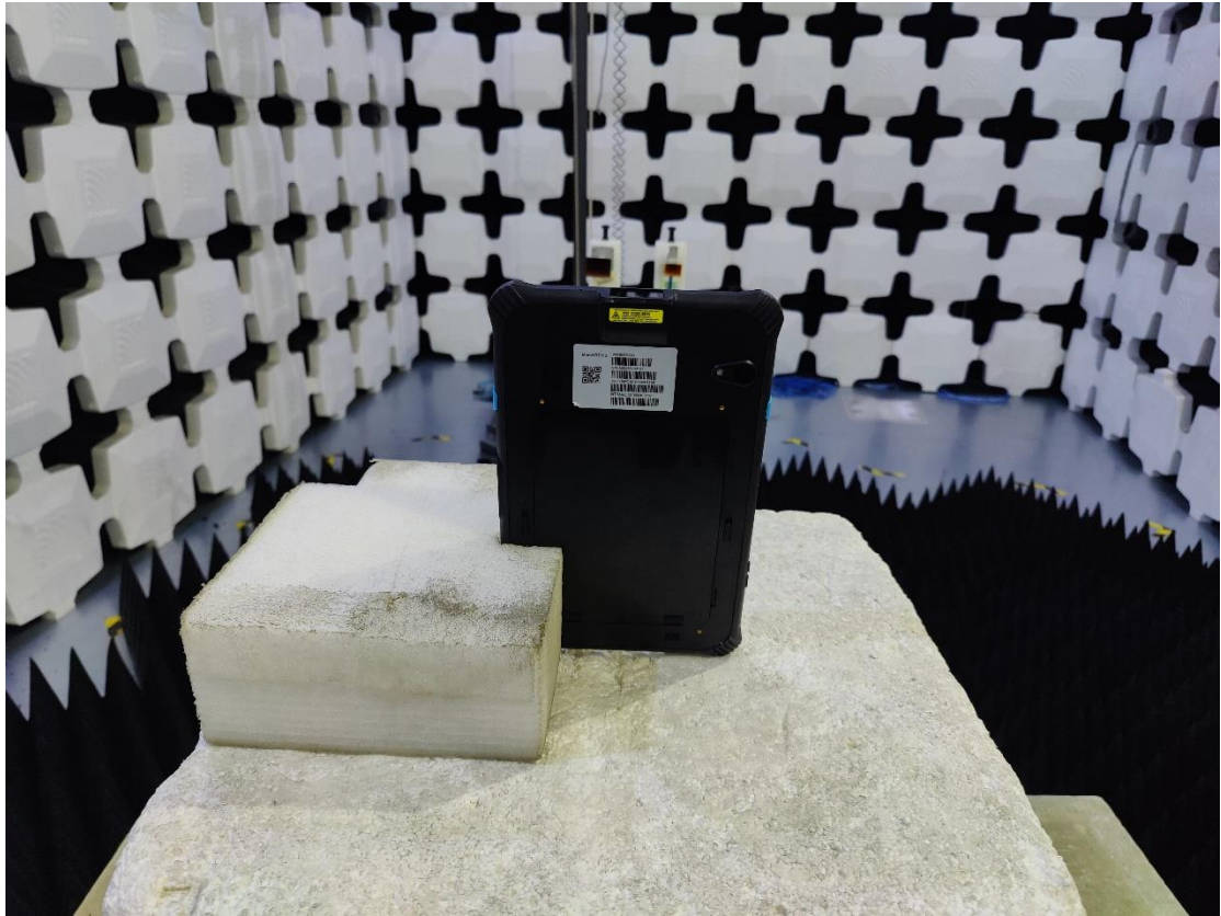
11. Radiated Emissions (Part 15C, 26.5GHz-40GHz)
