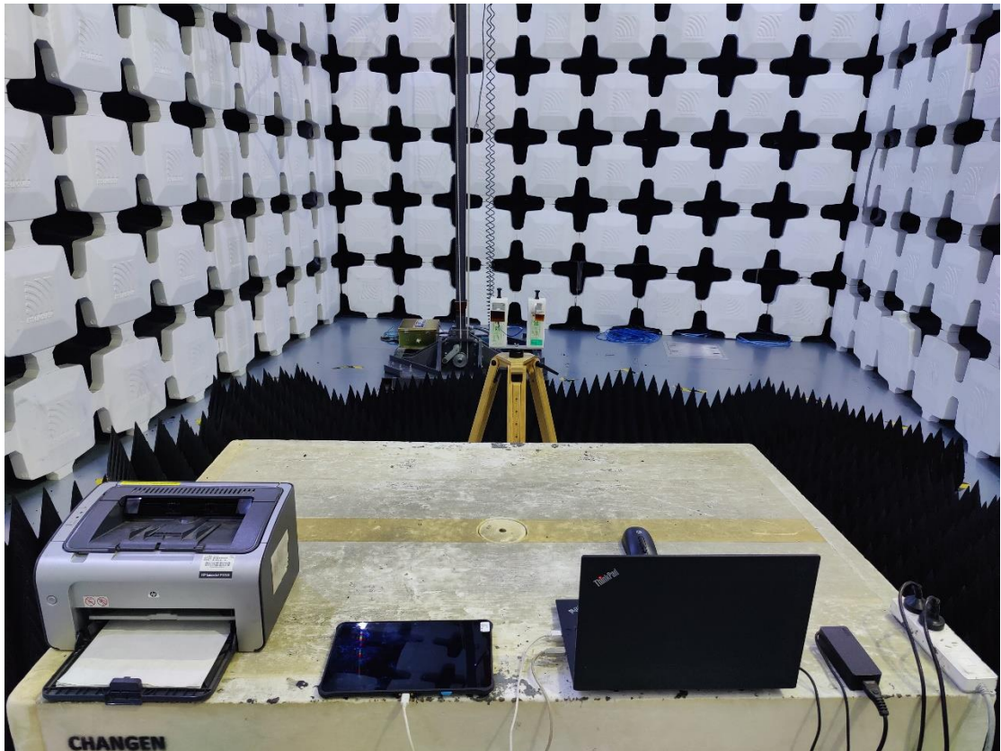
7. Radiated Emissions (Part 15B Data Transfer, 18GHz-26.5GHz)
