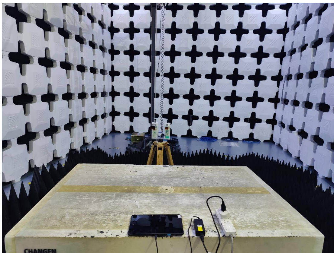
4. Radiated Emissions (Part 15B Camera, 26.5GHz-40GHz)
