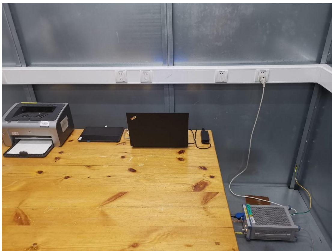
13. Conducted Emission (Part 15B, Data Transfer)
