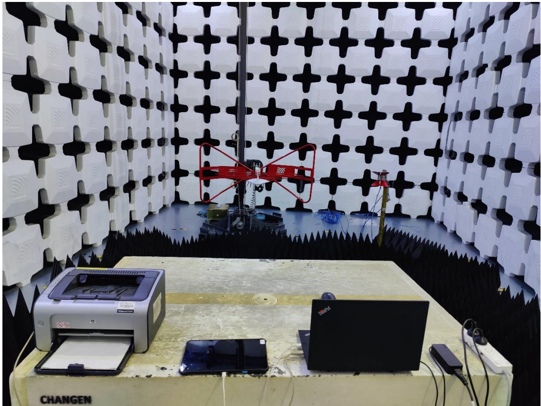
6. Radiated Emissions (Part 15B Data Transfer, 1GHz-18GHz)
