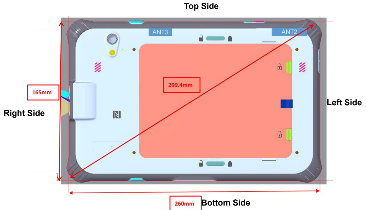
Picture 11.1 Antenna Locations (Back View)
