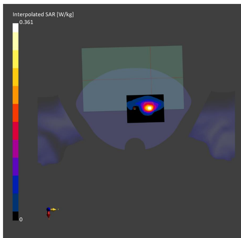
Fig. 1 Bluetooth Body
