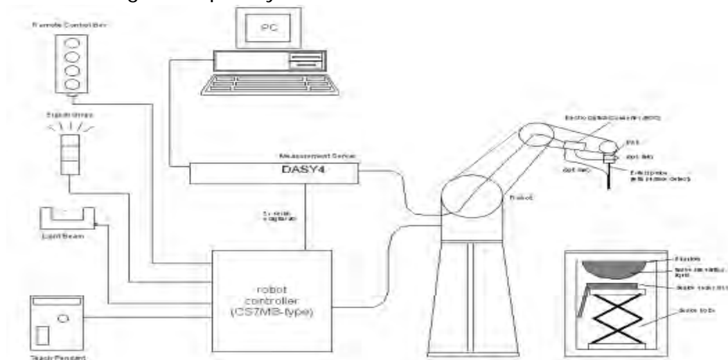
Fig.a The block diagram of SAR system
