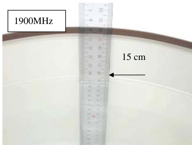
Fig.2.4 Photograph of the Tissue Simulant Fluid liquid depth 15cm for Right-head Side
