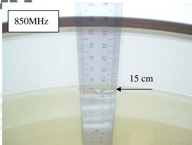
Fig.2.3 Photograph of the Tissue Simulant Fluid liquid depth 15cm for Body Side
