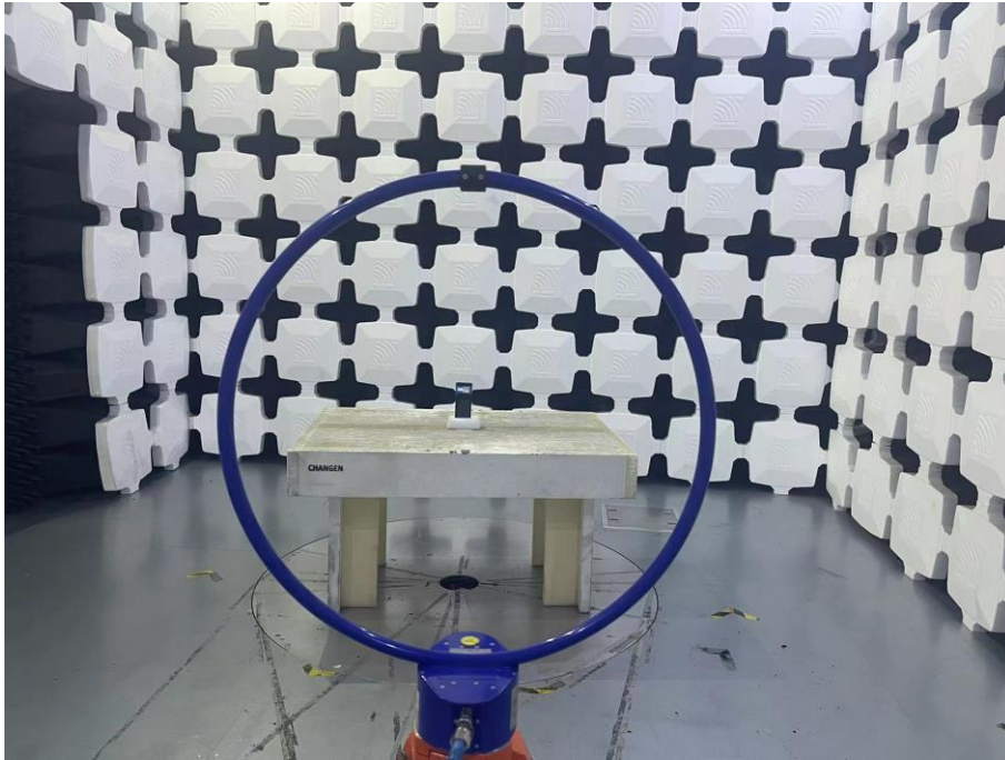
9. Radiated Emissions (Part 15C, 9kHz-30MHz)
