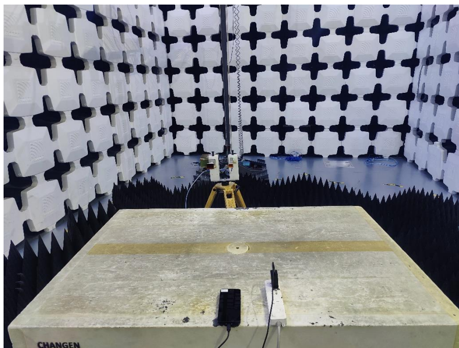
8. Radiated Emissions (Part 15B, Camera/Video Player/Scanner/GSM receiver/WCDMA receiver /LTE receiver/5G NR receiver, 26GHz-40GHz)
