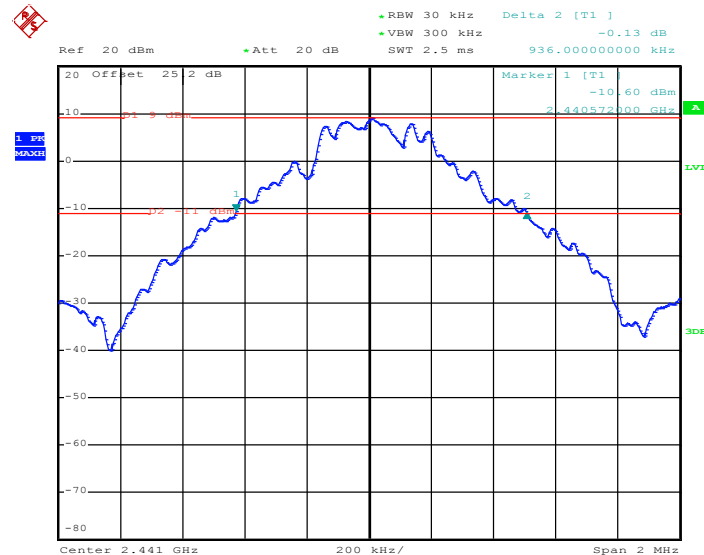
20 dB Bandwidth Plot on Channel 39
