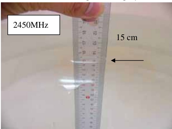
Fig.2 Photograph of the Tissue Simulant Fluid liquid depth 15cm for Flat (Body)
