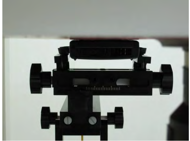
Fig.3 EUT front to flat phantom
