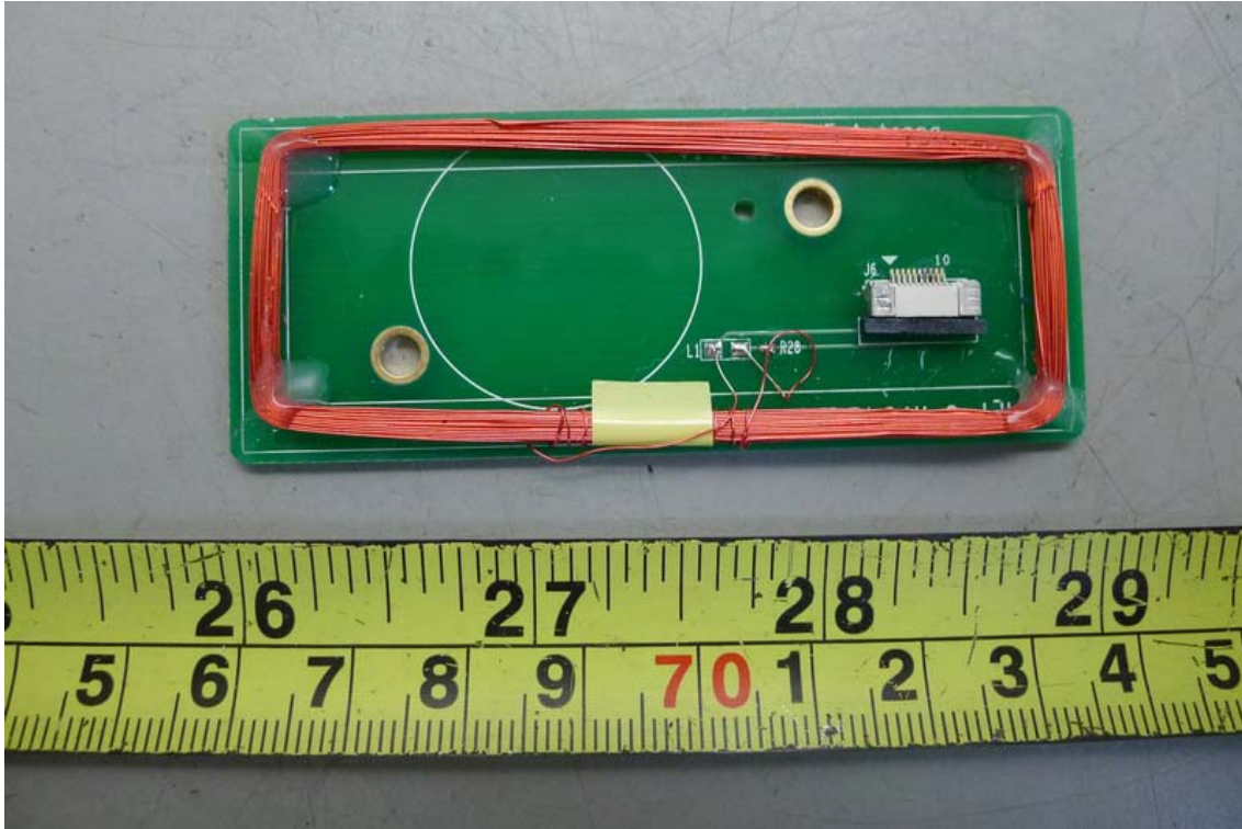
RFID Antenna: TC-680I-320-K
