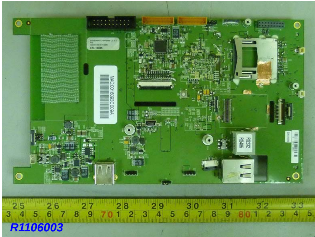
Model Name: MT650-APUEAG Main board
