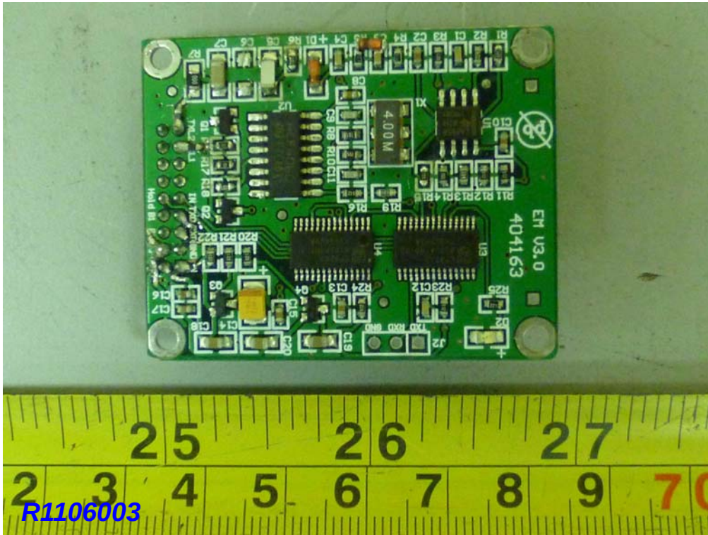
Model Name: MT650-AYUEAG 125 KHz Module (EM)
