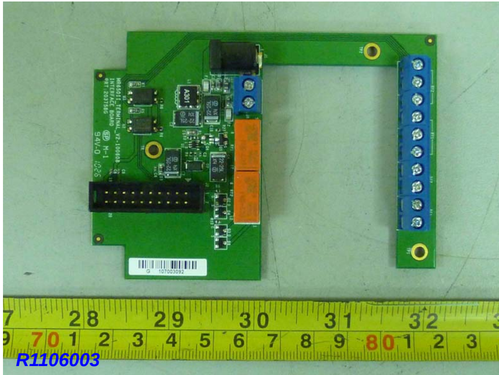
Model Name: MT650-AYUEAG Components board
