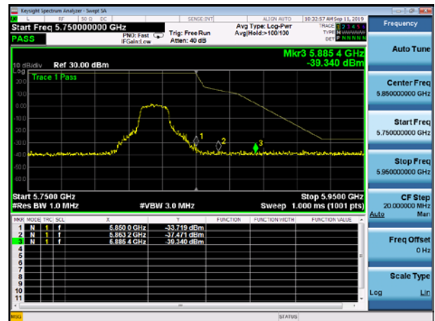
U-NII-3 Band Edge-802.11a(20MHz) ,5825MHz
