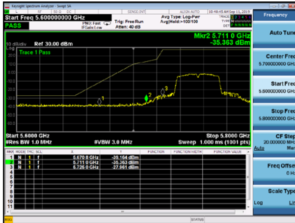
U-NII-3 Band Edge-802.11a(20MHz) ,5745MHz
