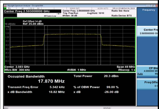
TDD41_MidRange_20_2593_Q16
