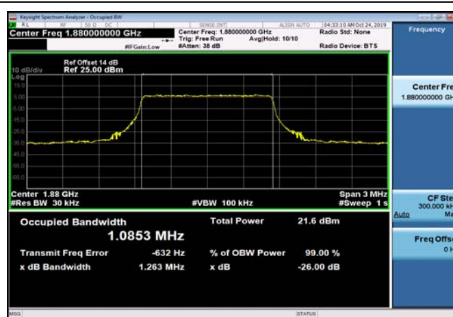
FDD02_MidRange_3_1880_Q16
