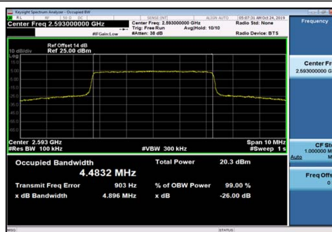
TDD41_MidRange_5_2593_Q16
