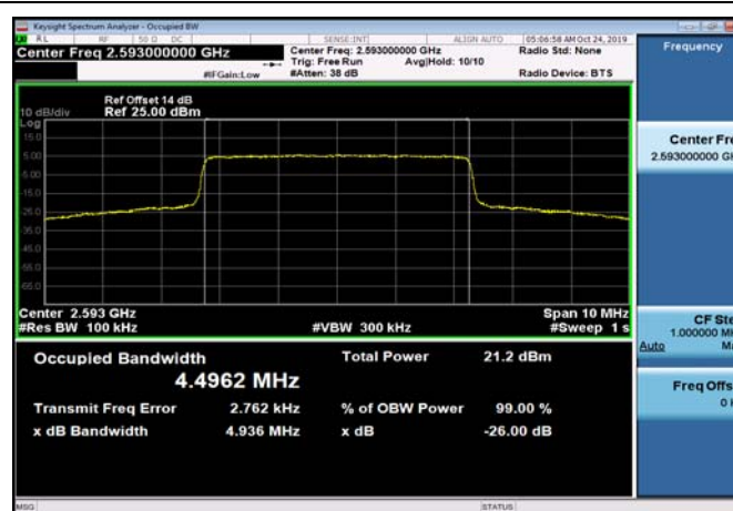
TDD41_MidRange_5_2593_QPSK
