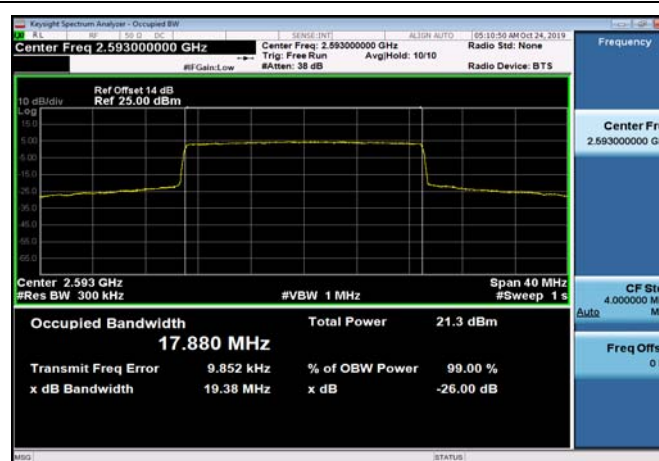
TDD41_MidRange_20_2593_QPSK
