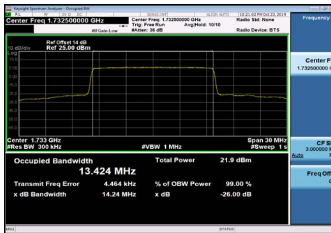
FDD04_MidRange_15MHz_1732.5MHz _QPSK
