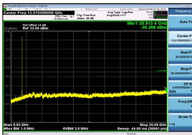
FDD02_HighRange_5MHz_30MHz~26GHz
