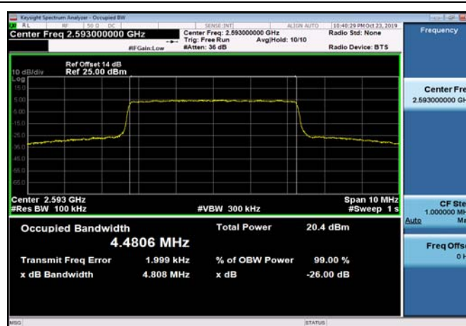
TDD41_MidRange_10MHz_2593MHz_Q16
