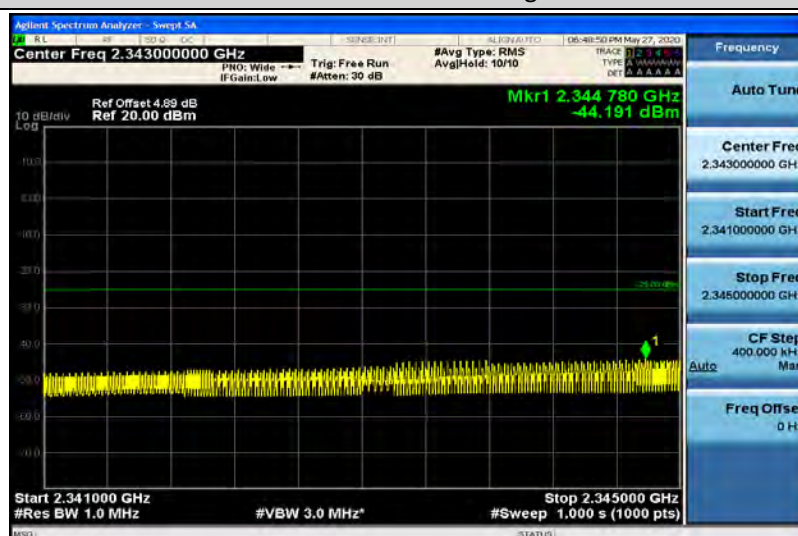
Band40-5MHz-16QAM-39175-1RB#24-Range10:2341~2345MHz
