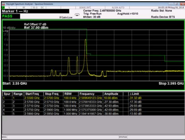
HighRange_FDD07_5MHz_2567.5_fullRB _HighQPSK
