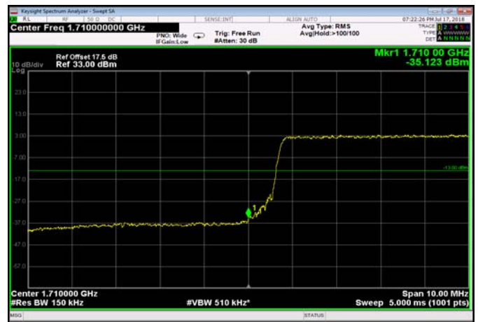
LowRange_FDD04_20MHz_1720_OneRB _low_Q16
