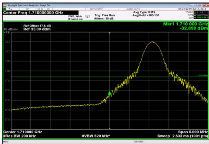
LowRange_FDD04_20MHz_1720_fullRB _LowQPSK
