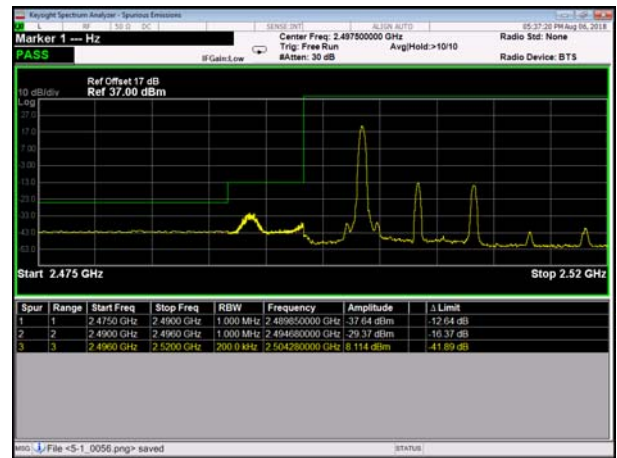
LowRange_FDD07_10MHz_2505_fullRB _LowQ16
