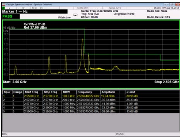
HighRange_FDD07_15MHz_2562.5_fullRB _HighQPSK
