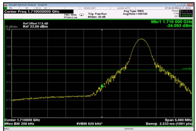
LowRange_FDD04_20MHz_1720_fullRB _LowQ16
