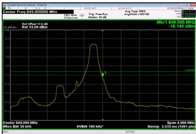
HighRange_FDD05_3MHz_847.5_fullRB _HighQPSK
