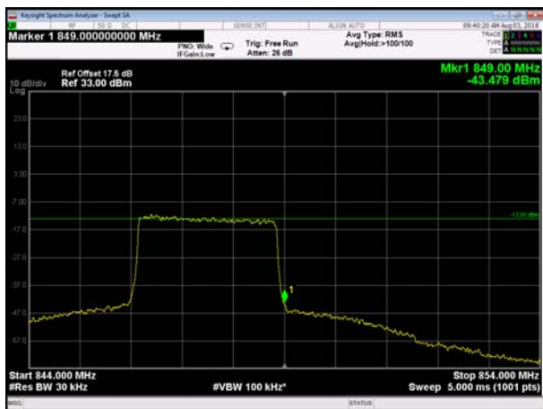
HighRange_FDD05_3MHz_847.5_fullRB _HighQPSK
