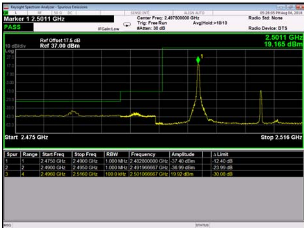
LowRange_FDD07_20MHz_2510_fullRB _LowQPSK
