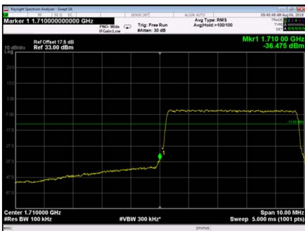
HighRange_FDD04_10MHz_oneRB _HighQPSK
