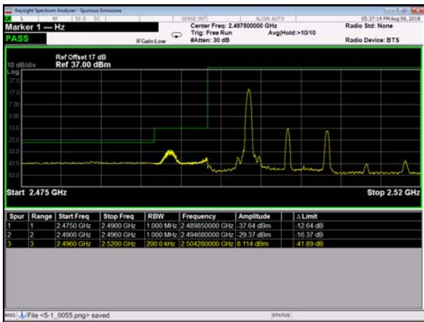
LowRange_FDD07_10MHz_2505_fullRB _LowQPSK
