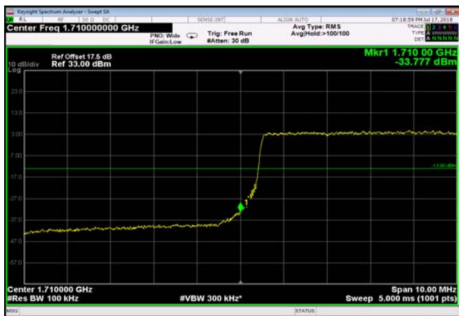
LowRange_FDD04_15MHz_1717.5_OneRB _low_QPSK
