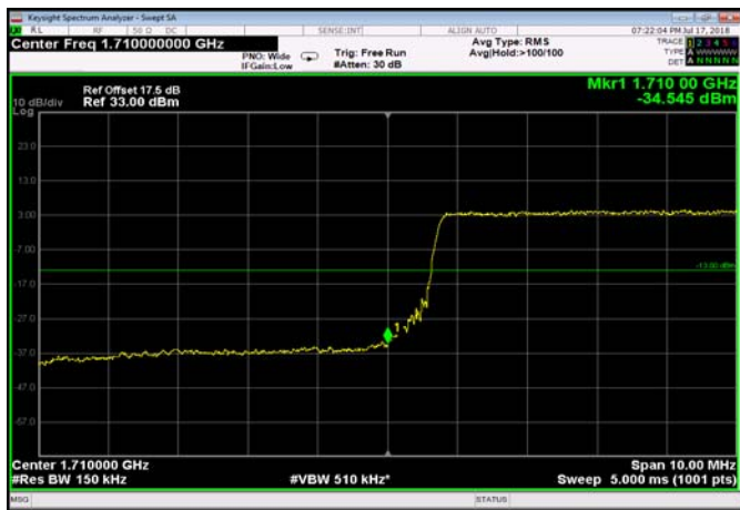
LowRange_FDD04_20MHz_1720_OneRB _low_QPSK
