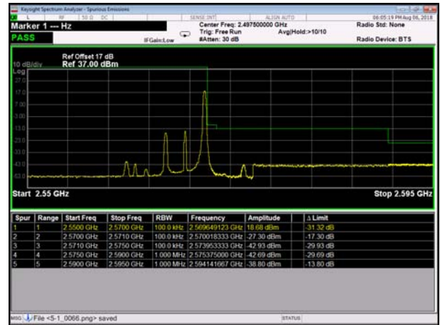
HighRange_FDD07_5MHz_2567.5_fullRB _HighQ16
