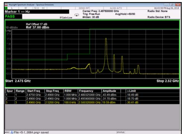
LowRange_FDD07_5MHz_2502.5_fullIRB _LowQ16
