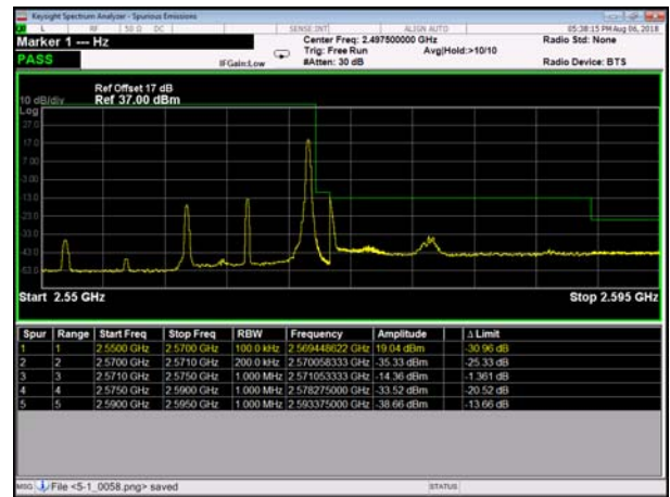
HighRange_FDD07_15MHz_2562.5_fullRB _HighQ16
