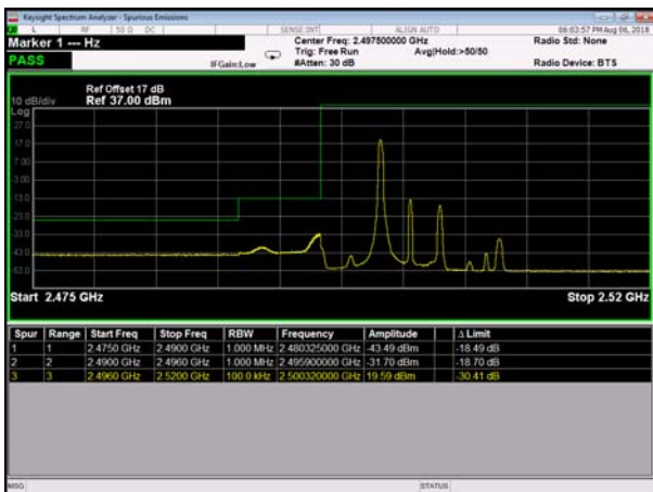
LowRange_FDD07_5MHz_2502.5_fullIRB _LowQPSK
